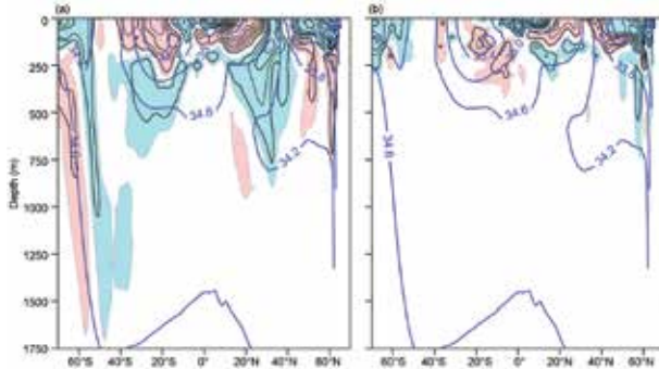
FIG. 3.14. Zonally averaged (a) 2014 salinity anomaly and (b) 2014 minus 2013 salinity for the Pacific Ocean. Blue shading represents negative (fresh) anomalies <-0.01 , red shading represents positive (salty) anomalies >0.01 . Anomalies are contoured at 0.02 intervals. Zonally averaged climatological mean salinity values (Antonov et al. 2010) are contoured (thick blue lines) at 0.4 intervals. All values are reported on the 1978 Practical Salinity Scale (PSS-78).
