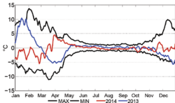
FIG. 2.5. Julian-day-of-year time series of the 2013 (blue) and 2014 (red) TLS temperature anomalies (°C) for the 60°–90°N latitude band. The daily minimum and maximum anomalies over the 1979–2014 period are shown as black lines.
