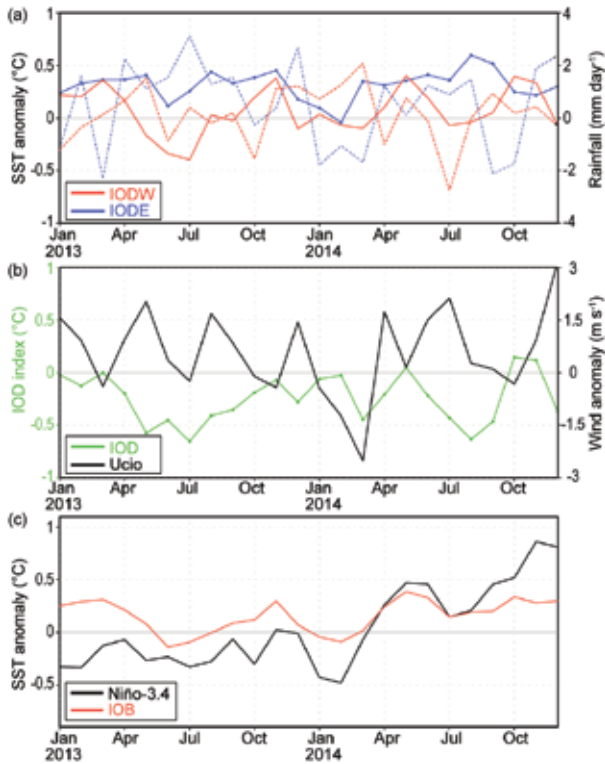
FIG. 4.41. (a) Monthly anomalies of SST (°C, solid lines) and precipitation (mm day -1 , dashed lines) in the eastern IO (IOE, 90°–110°E, 10°S–0°, blue lines) and western pole (IODW, 50°–70°E, 10°S–10°N, red lines) of IOD. (b) As in (a), but for the IOD index (measured by the SST difference between IODW and IOE, green line) and surface zonal wind anomaly (m s -1 ) in the central equatorial IO (Ucio, 70°–90°E, 5°S–5°N, black line). (c) As in (a), but for the SST anomalies in Niño-3.4 region (170°–120°W, 5°S–5°N, black line) and the tropical IO (IOB, 40°–120°E, 20°S–10°N, red line). Anomalies calculated relative to the 1982–2013 climatology. These are based on the NCEP optimum interpolation SST (Reynolds et al. 2002), monthly GPCP precipitation analysis, and JRA-55 atmospheric reanalysis (Ebita et al. 2011).
