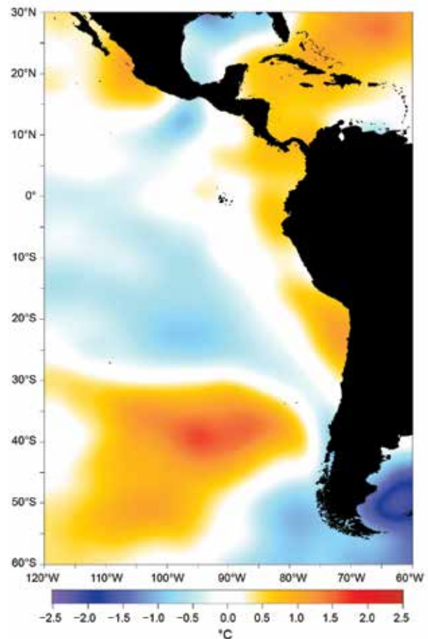
FIG. 7.11. Mean annual sea surface temperature anomalies ( ^\circ\text{C} ; 1971–2000 base period). Data source: NOAA/NCEP/EMC/CMB/GLOBAL Reyn_Smith Olv2. (Processed by CIIFEN, 2015.)
