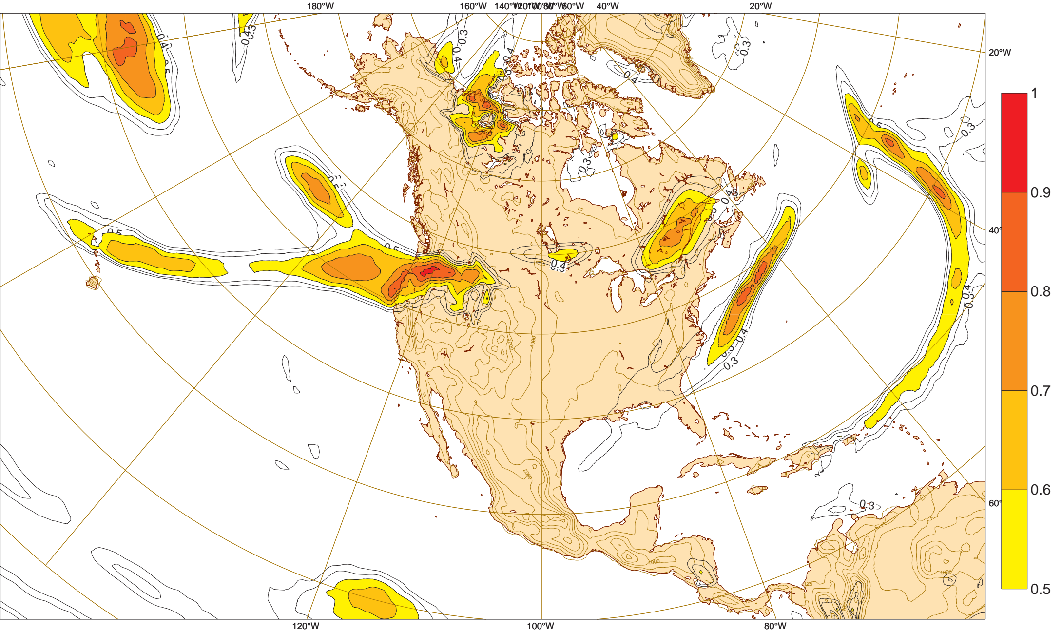
Monday 16 January 2012 00UTC ©ECMWF Extreme forecast index t+048-072 VT: Wednesday 18 January 2012 00UTC - Thursday 19 January 2012 00UTC Surface: Total precipitation index
