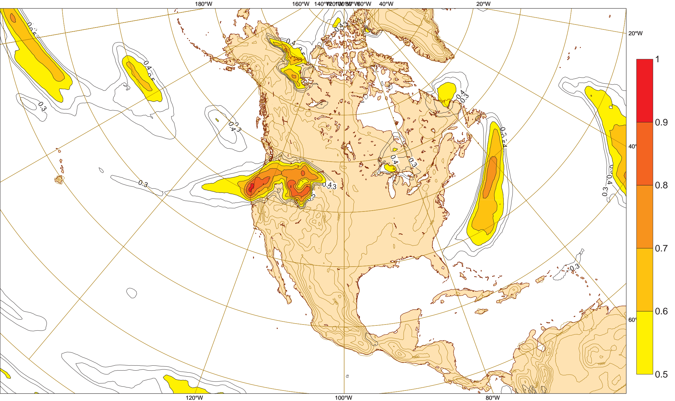
Monday 16 January 2012 00UTC ©ECMWF Extreme forecast index t+072-096 VT: Thursday 19 January 2012 00UTC - Friday 20 January 2012 00UTC Surface: Total precipitation index
