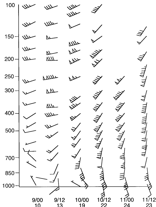
FIG. 17. Time–height cross section of sounding winds from Anchorage, Alaska, 9–11 October 1986. Full barbs are 10 kn ( 5.1 \text{ m s}^{-1} ) and half barbs are 5 kn ( 2.55 \text{ m s}^{-1} ). The numbers below the cross section indicate sounding date and time (UTC) and precipitable water in mm.
