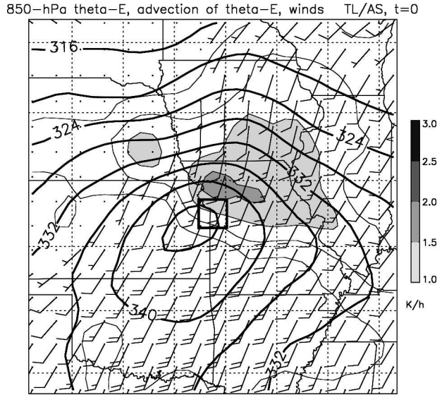
FIG. 15. Composite of 850-hPa equivalent potential temperature (K; thick lines), equivalent potential temperature advection (thin gray lines) \theta_e , and winds (kt; conventional plotting) at the peak rainfall time for TL/AS MCS extreme rain events. Advection contour interval is 0.5 K h^{-1} , and values greater than 1.0 K h^{-1} are shaded. Map projection is the same as in Fig. 11.
