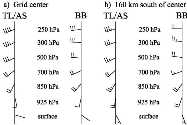
FIG. 13. Composite wind profile at (a) the grid center and (b) four grid points (~160 km) south of the center for TL/AS and BB MCS extreme rain events at the peak rainfall time. Wind bars are plotted conventionally in kt. Recall that the grid has been rotated for some cases, so 160 km south of the center may physically represent a distance east or west of the center, but still reflects the inflowing air.
