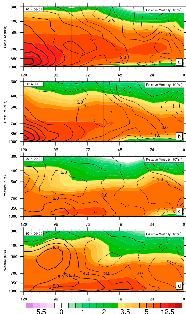
FIG. 10. Ensemble mean forecast evolution of the vertical profile of relative vorticity around each ensemble trough center (shading; 10^{-5} \text{ s}^{-1} ). The ensemble mean error is shown as contours ( 10^{-5} \text{ s}^{-1} ). Forecast hour (x axis) increases from right to left, as the trough moves east to west. The vertical black line denotes the trough passage over the coast. Each panel shows a different initialization time displayed in the top-left corner.
