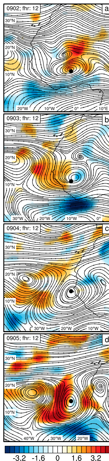
FIG. 14. Trough-relative streamlines layer averaged between 900 and 700 hPa. Shading shows sign and significance of the ensemble-based 42-h precipitation forecast sensitivity to layer average moist static energy ( \sigma ). Positive shading denotes increased moist static energy at that location is significantly correlated to increased precipitation in the trough at hour 42.
