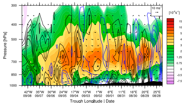
FIG. 3. Vertical profile evolution for 6-hourly variables averaged over 300 km around the trough center. Relative vorticity (background shading), the 6-hourly change in specific humidity [blue (black) contours for positive (negative) 0.5 g kg ^{-1} day ^{-1} ], and wave-relative zonal and meridional wind (vectors; the top of the plot represents north for meridional wind). Surface intersecting isobars are masked. Vertical line at 0600 UTC 4 Sep represents troughs transit over the coast.
