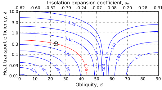
Figure 4. Contour plot of the minimum radiative forcing q_{free} for which an ice-free solution exists, as a function of obliquity and heat transport efficiency. A logarithmic scale is used for \delta since it may vary over orders of magnitudes. For comparison to Earth-like planets, the red contour shows q = 1.2 (the present-day value based on (11d)), and the Earth symbol (circle with cross) indicates q_{free} for \beta = 23.45^\circ , \delta = 0.31 from (21). The fact that this point sits on the red line indicates that present-day Earth is near a radiative forcing that supports an ice-free state according to this model.
