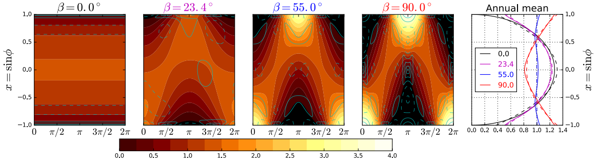
Figure 2. Spatiotemporal distribution of daily-average insolation for four different obliquity values \beta . Colored contours show the normalized daily-average insolation s(x, \tau) (unit global, annual mean) with x = \sin \phi an area-weighted latitude and \tau = 2\pi t/t_{year} a seasonal time angle. For the present-day value \beta = 23.45^\circ we use realistic present-day eccentricity and precessional parameters. For the other three cases ( \beta = 0^\circ, 55^\circ, 90^\circ ) the eccentricity is set to zero. The thin contours indicate error of the truncated series fit (2), (3) (contour interval is 0.1, negative contours dashed). The right-most panel shows the annual mean insolation for the four obliquity values (solid), along with the truncated series fit \bar{s}(x) = 1 + s_{20}P_2(x) (dashed). These illustrate the reversal of the annual-mean insolation gradient at the critical value \beta \approx 55^\circ .
