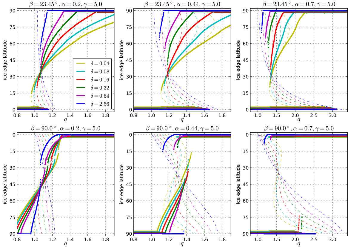
Figure 10. Same as Fig. 9 but for the “intermediate water depth” regime, \gamma = 5 .
