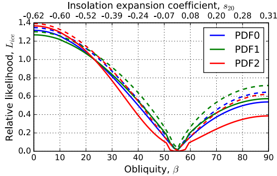
Figure 7. Estimates of the relative likelihood L_{ice} of finding a planet with stable finite ice cover – either ice caps (for low obliquity) or ice belt (for high obliquity). The curves show L_{ice} calculated from (32) and (33) and for three different forms of probability density h_{planet} as described in the text, and normalized to a value of 1 at Earth’s obliquity of 23.45^\circ . Dashed curves include all possible stable ice edges. Solid curves exclude inaccessible stable states using (34).
