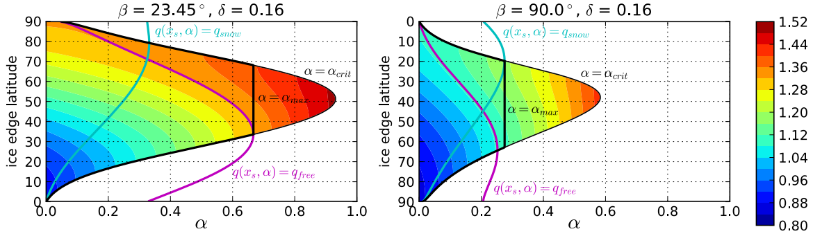
Figure 6. Graphical illustration of the method for excluding inaccessible stable states. In colors we contour q(x_s, \alpha) from (25) for the stable region bounded by \alpha_{crit} from (30). Magenta curve is the implicit solution of q(x_s, \alpha) = q_{free} – the latitude to which the ice edge would jump in an unstable transition from ice-free conditions. Cyan contour is the implicit solution of q(x_s, \alpha) = q_{snow} – the analogous ice edge latitude resulting from unstable transitions from the Snowball state. \alpha_{warm} in (34) is the intersection of the magenta curve with \alpha_{crit} . For \alpha > \alpha_{warm} , transitions from ice-free conditions would result directly in a Snowball. Similarly, \alpha_{cold} is the intersection of the cyan curve with \alpha_{crit} , giving the maximum \alpha for which transitions from Snowball to stable ice edge are possible. The thick black contour illustrates \alpha_{max} from (34). Inaccessible stable states lie between \alpha_{max} and \alpha_{crit} .
