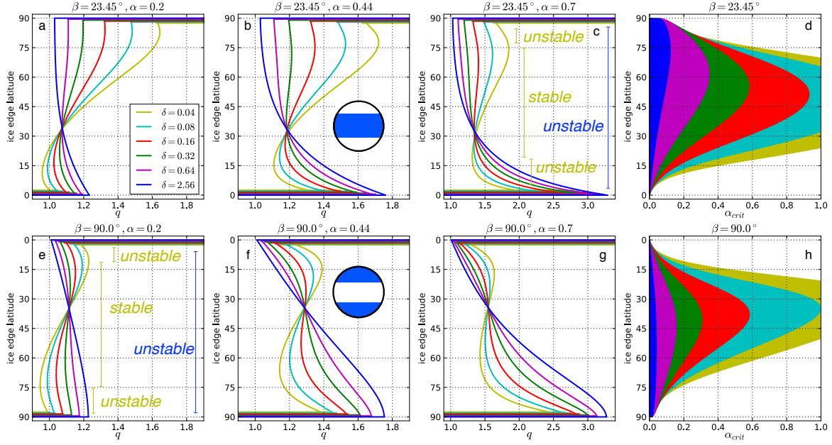
Figure 5. The radiative forcing q required as a function of ice edge latitude \arcsin(x_s) , for various parameter values. Upper row: Earth-like obliquity \beta = 23.5^\circ ; ice cap is poleward of the indicated latitude. Lower row: \beta = 90^\circ , warmest temperatures at the poles, ice belt is equatorward of the indicated latitude. The latitude axis is flipped so that the icy region is above the indicated latitude in all cases. Panels a-c and e-g show q(x_s) computed from (25) for several different values of \delta ranging from 0.04 to 2.56. Stable equilibria exist wherever the graphs slope upward to the right. Panels d and h show the ranges of possible stable ice edges as a function of the albedo feedback parameter \alpha . For a given \delta value, stable ice edges are possible only within the shaded region \alpha < \alpha_{crit} .
