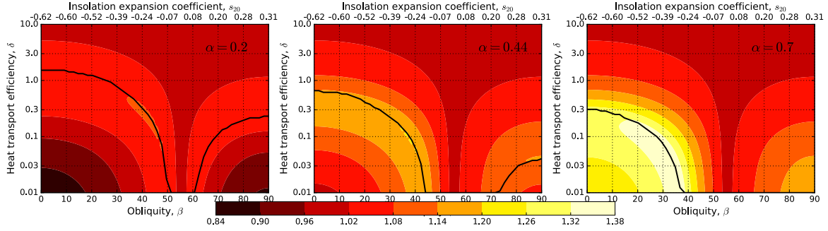
Figure 8. Contour plots of q_{hab} , the minimum q required for a non-Snowball climate. q_{hab} , defined by (36), is contoured for fixed albedo contrast parameter \alpha as a function of obliquity and heat transport efficiency \delta . Darker colors indicate smaller q_{hab} , i.e. a planet less prone to the Snowball catastrophe. The black contours indicate values of \delta above which q_{hab} = q_{free} , i.e. the Snowball bifurcation occurs directly from the ice-free state. For \delta below this line, the bifurcation occurs from a stable partially ice-covered state.
