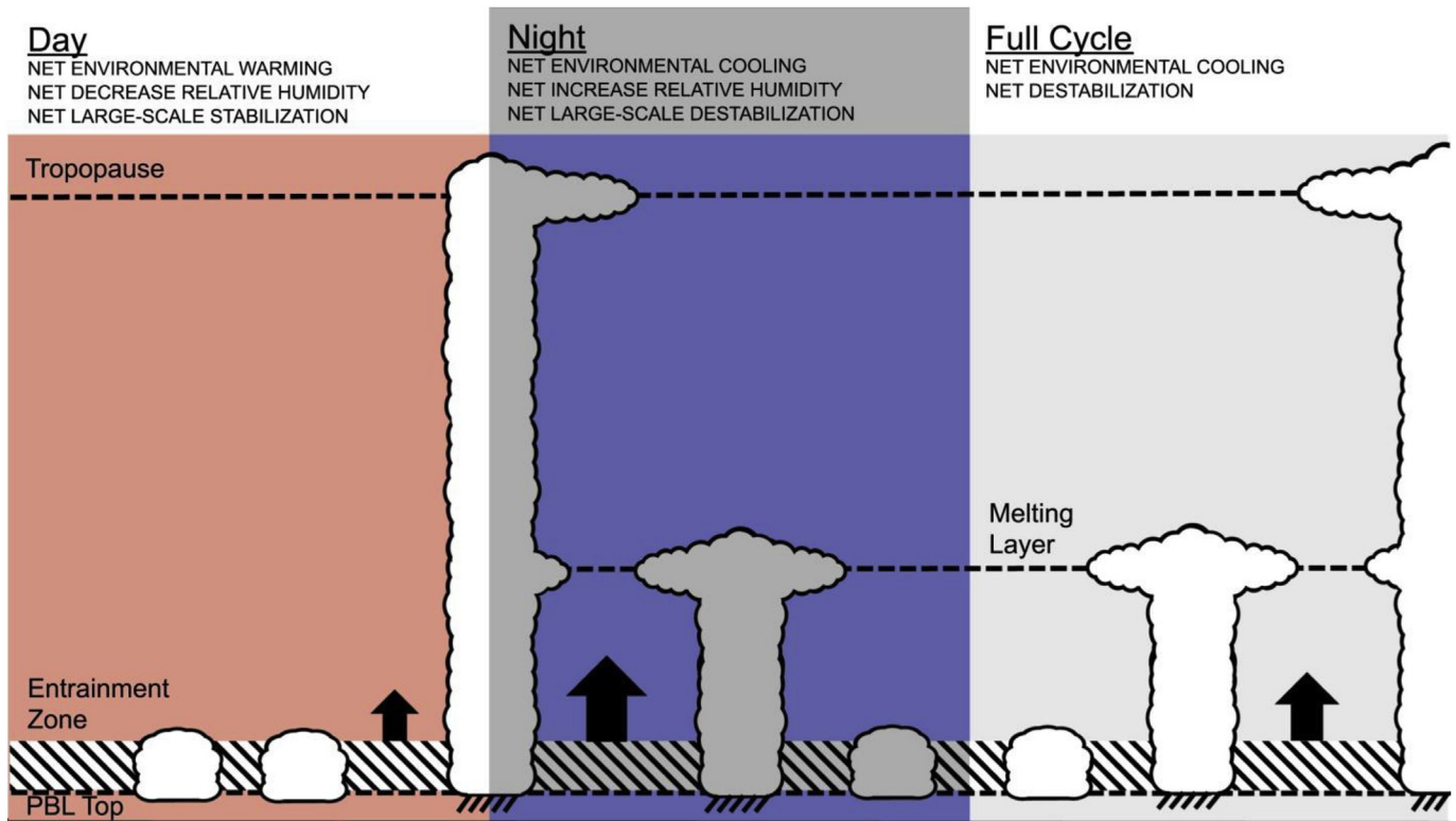
Fig. 16. Schematic depiction of the diurnal radiation cycle impact on the clear-air local and large-scale environment for the genesis of Hurricane Karl (2010) during the first 24 h of a simulation. The red (blue) background shading of day (night) indicates net clear-air large-scale environmental heating (cooling). Arrows indicate the relative magnitude of the local-environment clear-air net radiative cooling (solid) for the entrainment zone. Adapted from Melhauser and Zhang (2014). © American Meteorological Society. Used with permission.
