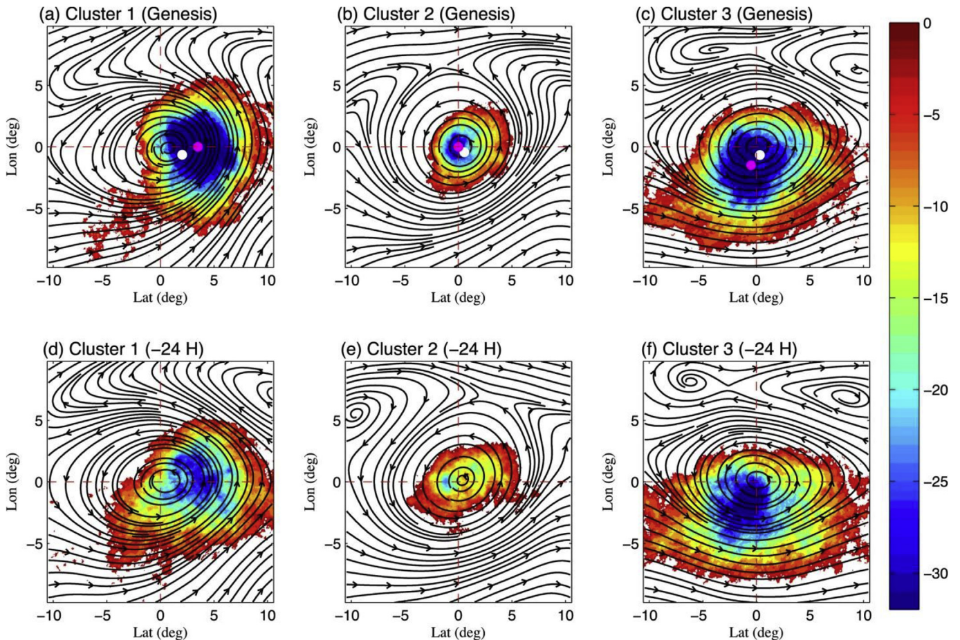
Fig. 6. Composite mean of infrared brightness temperature ( ^{\circ}\text{C} ) superimposed on 700-hPa wave-relative streamlines for three distinct convective clusters embedded in different environments at (a)–(c) the time of genesis and (d)–(f) 24 h prior to genesis. The white dots in (a)–(c) represent the composite mean genesis location for each cluster, and the magenta dots are the convection centers. Reproduced from Wang (2018). © American Meteorological Society. Used with permission.
