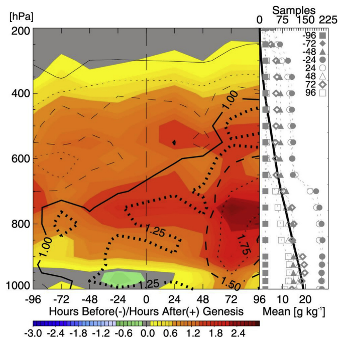
Fig. 12. Composite water vapor mixing ratio anomaly (color shaded) of all dropsondes within 3° of the 850-hPa vorticity maximum center for all genesis cases; black contours are standard deviation. Number of samples (gray) at each time and the mean profile (black) are indicated on the right. Reproduced from Zawislak and Zipser (2014b). © American Meteorological Society. Used with permission.
