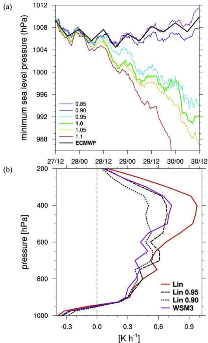
Fig. 14. (a) Minimum sea level pressure (hPa) for simulations that used the Purdue–Lin microphysics scheme in which the diabolic heating rate was multiplied by a factor ranging from 0.85 to 1.1. The minimum sea level pressure from the ECMWF analysis (black) is shown for reference. (b) Vertical profiles of the average diabolic heating rate ( \text{K h}^{-1} ) for the period 1800 UTC 27 August–0600 UTC 28 August for the Lin simulation (red line), the WSM3 simulation (purple line), and for simulations that used the Purdue–Lin microphysics scheme in which the diabolic heating rates were multiplied by a factor of 0.95 (long dashed line) and 0.90 (short dashed line). Reproduced from Penny et al. (2016). © American Meteorological Society. Used with permission.
