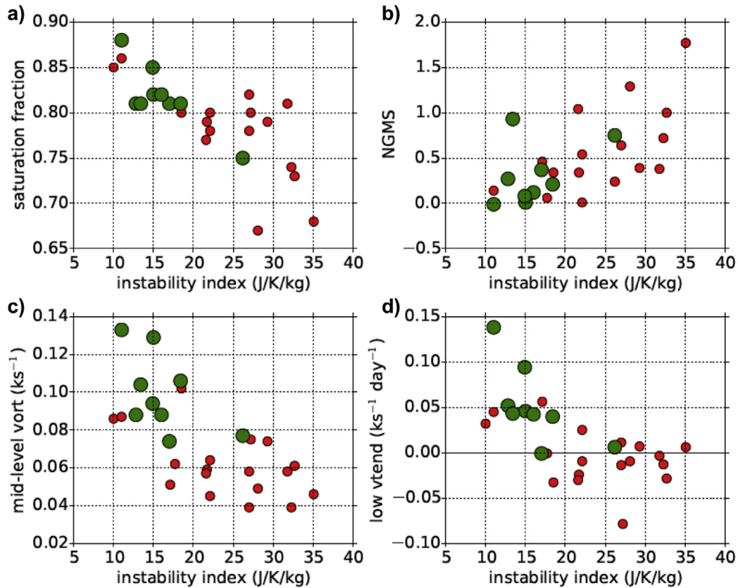
Fig. 13. (a) Saturation fraction, (b) normalized gross moist stability, (c) mid-level mean absolute vorticity, and (d) low-level mean absolute vorticity versus instability index (increasing values indicate greater moist convective instability between the lower and middle troposphere) for tropical disturbances observed by field campaigns in the western North Pacific (TCS08) and the North Atlantic (PREDICT). The cases represented by large green dots intensified into tropical storms within 48 h of the observations, while cases represented by small red dots did not. Adapted from Raymond et al. (2014).
