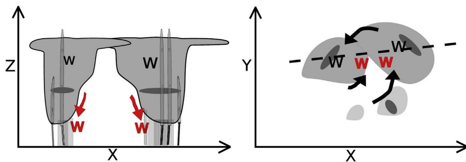
Fig. 11. Schematic of warm-core development in genesis. (left) Vertical cross sections: the dark horizontal shading represents the melting level within mesoscale convective systems. (right) Plan views with the cross-section location marked with the dashed line; dark shading represents heavy convective rainfall. Areas of mesoscale subsidence are indicated with red arrows, and associated warming by the red “W”s. Upper-level warming in the anvil is indicated by the black “W”s. Adapted from Kerns and Chen (2015). © American Meteorological Society. Used with permission.
