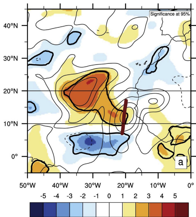
Fig. 9. Mean composite total precipitable water (mm) differences for favorable developing waves vs. favorable nondeveloping waves (shading). Contours represent the composite favorable developing waves. The shading and contour intervals are equivalent. The thick red line depicts the mean trough line of all included waves. The thick black contour encompasses the regions that are statistically significant at greater than 95%. Adapted from Brammer and Thorncroft (2015) . © American Meteorological Society. Used with permission.
