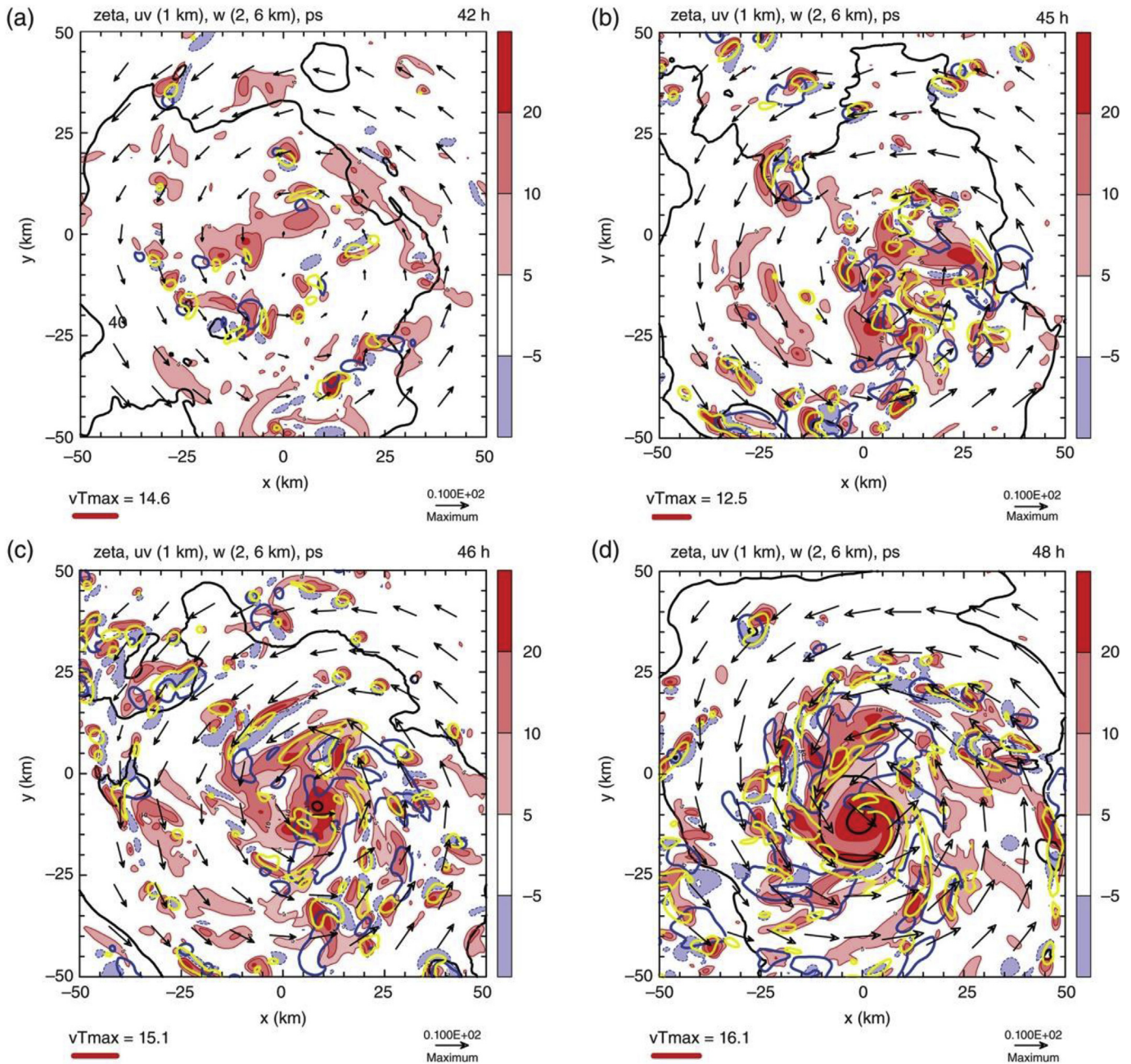
Fig. 8. Horizontal cross-sections of relative vertical vorticity ( \times 10^{-4} \text{ s}^{-1} , color shading) and wind vectors at a height of 1 km for a genesis simulation, with 1 \text{ m s}^{-1} contour of vertical velocity at heights of 2 km (blue) and 6 km (yellow). Also shown are surface pressure (black contours every 2 hPa). The wind vectors are in relation to the maximum reference vector at the bottom right, while on the bottom left the maximum total wind speed in the domain plotted is given in \text{m s}^{-1} . The times shown are: (a) 42 h, (b) 45 h, (c) 46 h, (d) 48 h. Reproduced from Kilroy et al. (2017b).
