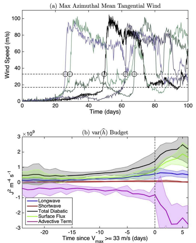
Fig. 15. Five-member ensemble of genesis in RCE simulations. (a) The evolution of the maximum azimuthal-mean tangential wind for each ensemble member. The dashed lines indicate wind speeds of 17 \text{ m s}^{-1} and 33 \text{ m s}^{-1} . The circles indicate the first time the wind speed reaches 33 \text{ m s}^{-1} . (b) The contributions to the growth rate of column-integrated frozen moist static energy variance for the ensemble members shown in (a), where the solid line is the ensemble mean and the shading indicates the standard deviation. The ensemble members are aligned at the times indicated by the circles in (a), which is defined as time 0 on the time axis in (b). Reproduced from Wing et al. (2016). © American Meteorological Society. Used with permission.
