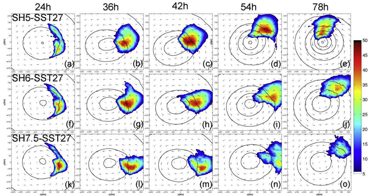
Fig. 5. Sea-level pressure (contour), surface wind (vector), and maximum reflectivity (shading) at 24, 36, 42, 54, and 78 h for simulations with (top row) 5 \text{ m s}^{-1} , (middle row) 6 \text{ m s}^{-1} , and (bottom row) 7.5 \text{ m s}^{-1} of westerly shear. All simulations have a sea surface temperature of 27^\circ \text{C} . Reproduced from Tao and Zhang (2014) .
