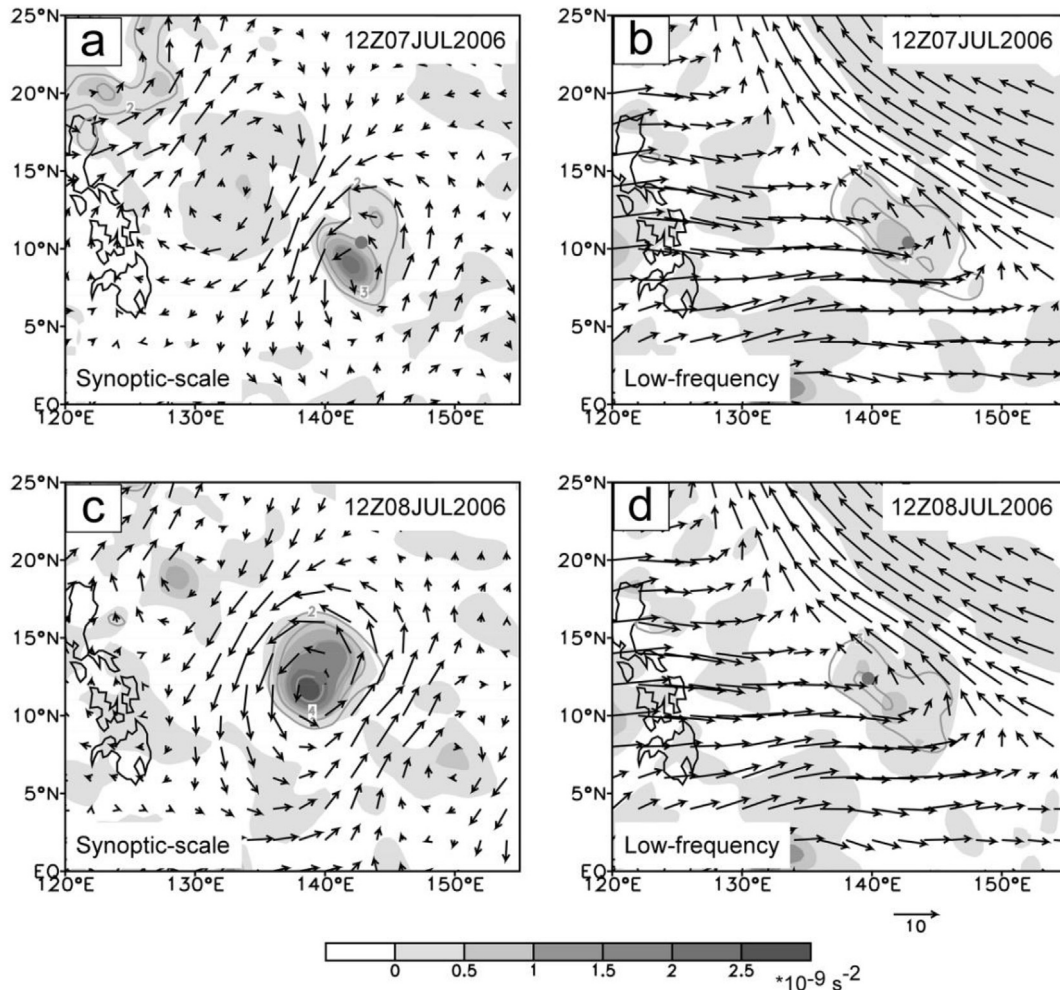
Fig. 3. (a),(c) The 850-hPa synoptic-scale and (b),(d) low-frequency relative vorticity (contours, 10^{-5} \text{ s}^{-1} ), Okubo–Weiss parameter (shaded, 10^{-9} \text{ s}^{-2} ), and winds (vectors, \text{m s}^{-1} ) at (a),(b) 1200 UTC 7 July and (c),(d) 1200 UTC 8 July 2006, with dots indicating the tropical disturbance center associated with Typhoon Bilis. Reproduced from Zong and Wu (2015b). © American Meteorological Society. Used with permission.
