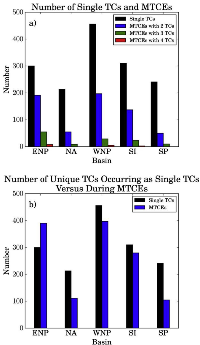
Fig. 2. Number of (a) single tropical cyclones and MTCEs with two, three, and four tropical cyclones and (b) uniquely named tropical cyclones occurring as single tropical cyclones vs. during MTCEs at any point during their lifetime within the eastern North Pacific (ENP), North Atlantic (NA), western North Pacific (WNP), South Indian (SI), and South Pacific (SP). Reproduced from Schenkel (2017). © American Meteorological Society. Used with permission.
