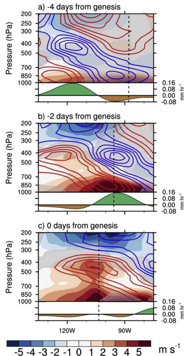
Fig. 1. Composite longitude–height cross sections of semi-Lagrangian total zonal wind (shading) and Kelvin-filtered zonal wind anomalies (contours) averaged 0^{\circ} – 10^{\circ}\text{N} for (a) four, (b) two, and (c) zero days before genesis. Values that are not 95% statistically significantly different from climatology are grayed out. Contours are drawn every 0.2 \text{ m s}^{-1} with westerlies in red and easterlies in blue. Line graphs show the associated Kelvin-filtered rainfall anomalies averaged 0^{\circ} – 10^{\circ}\text{N} . Longitudes are relative to genesis and are shown for reference only. Vertical dashed line identifies the estimated easterly wave trough. Reproduced from Schreck (2016) . © American Meteorological Society. Used with permission.
