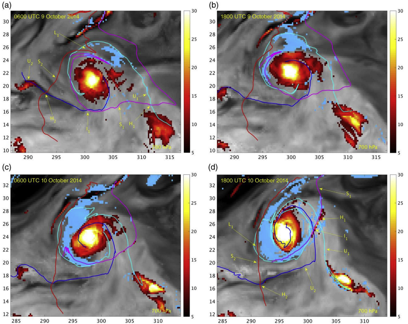
Fig. 10. Lagrangian flow topology (stable manifolds: magenta and red outlines, unstable manifolds: cyan and blue outlines), Lagrangian vorticity field (hot colors; dimensionless), the shearing regions of the Lagrangian Okubo-Weiss field (cool colors), and the equivalent potential temperature field (gray shading) at 700 hPa for Hurricane Fay during the development period at (a) 0600 UTC and (b) 1800 UTC on 9 October, and (c) 0600 UTC and (d) 1800 UTC on 10 October 2014. Reproduced from Rutherford et al. (2018).
