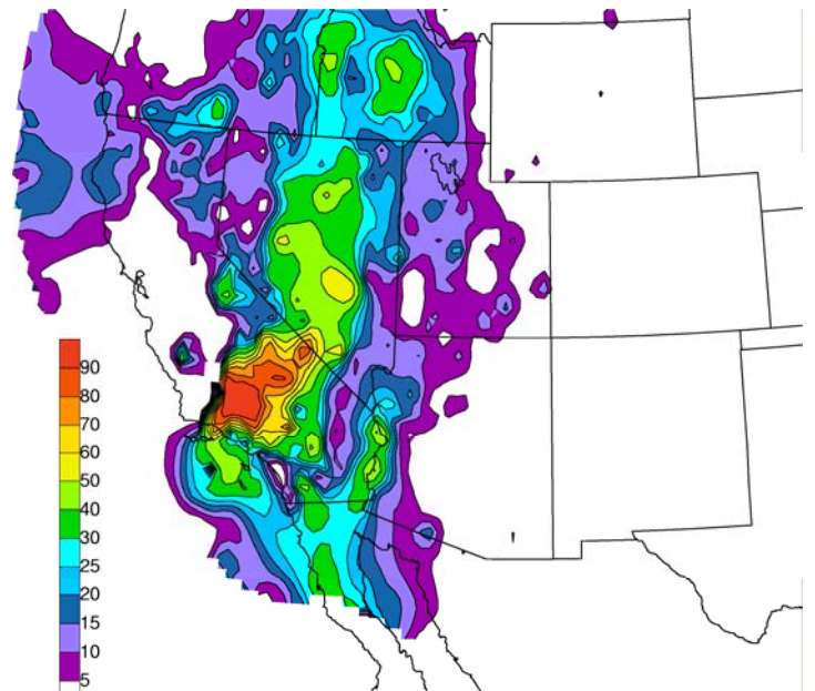
H 10 1959 Warm Season Precip Contribution
