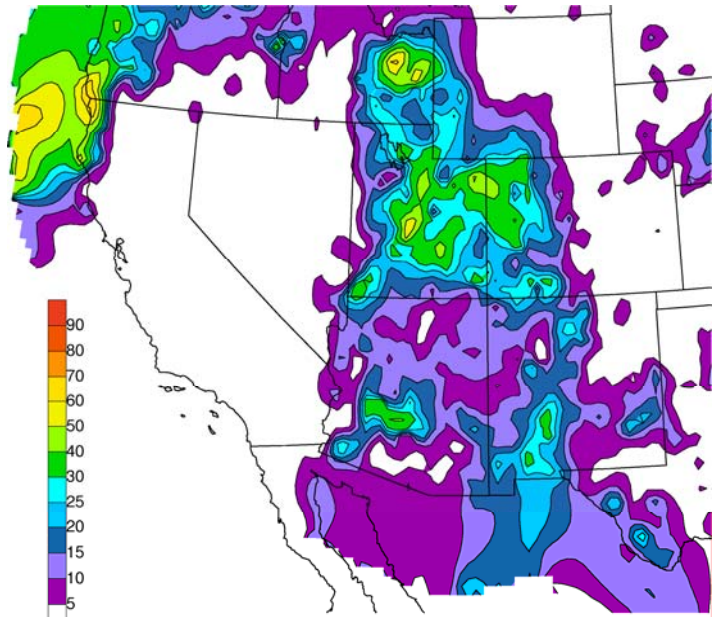
TS 10 1958 Warm Season Precip Contribution
