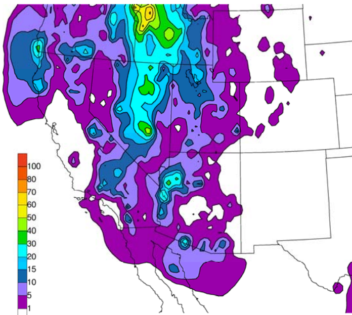
H 10 1959 Total Precipitation (mm) 11-15 September
