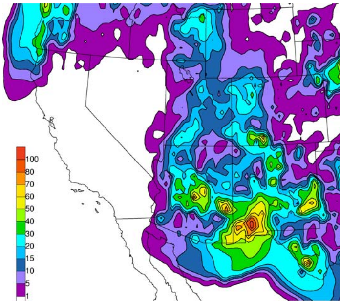
TS 10 1958 Total Precipitation (mm) 10-14 September
