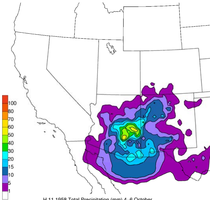
H 11 1958 Total Precipitation (mm) 4-6 October
