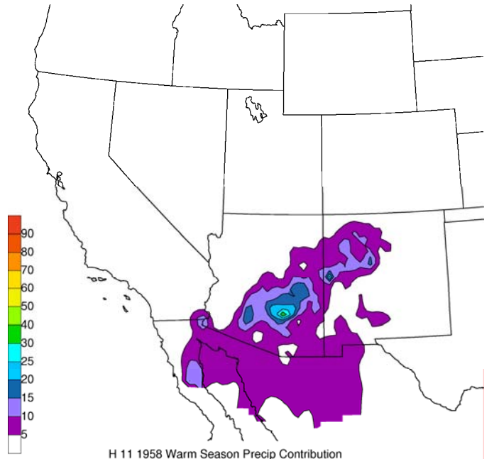
H 11 1958 Warm Season Precip Contribution
