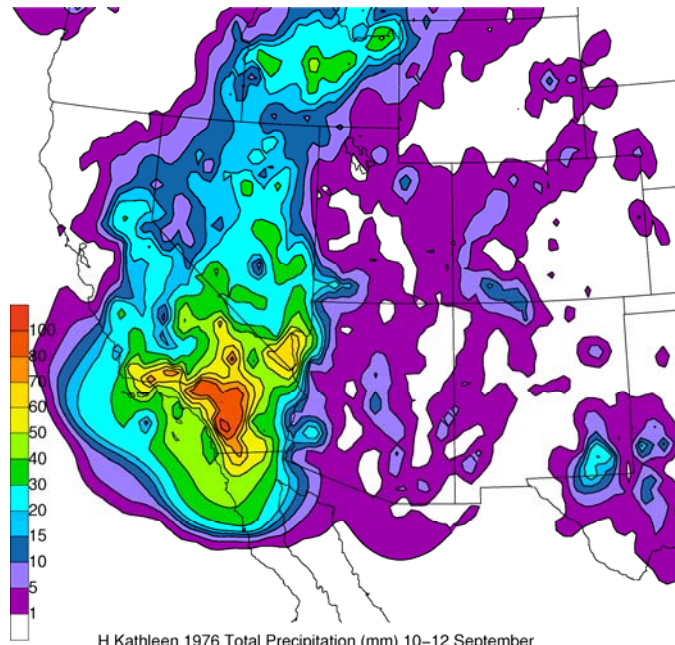
H Kathleen 1976 Total Precipitation (mm) 10-12 September
