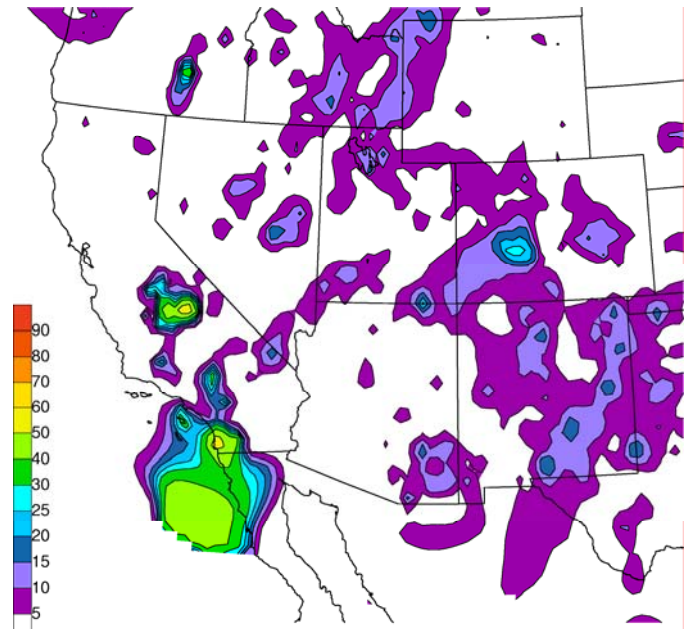
H Hyacinth 1972 Warm Season Precip Contribution
