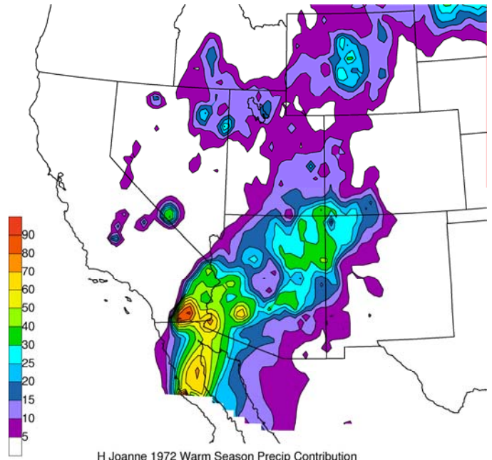
H Joanne 1972 Warm Season Precip Contribution
