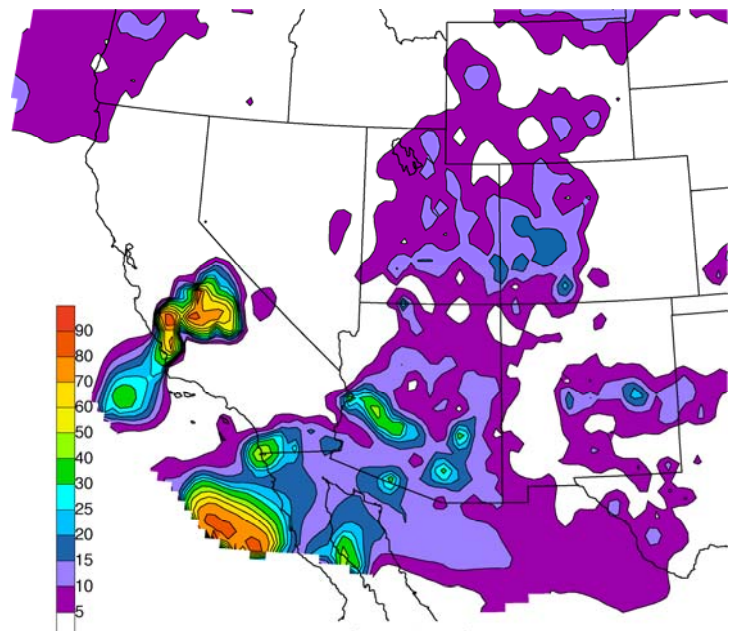
H Heather 1977 Warm Season Precip Contribution
