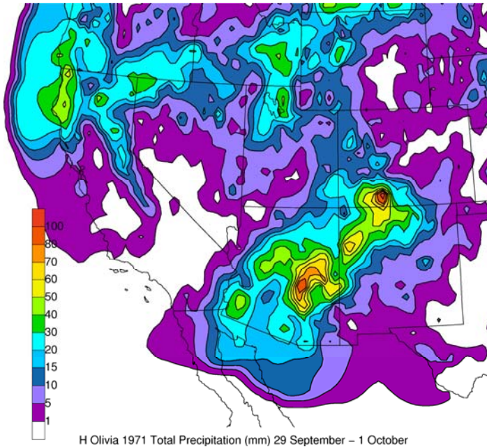
H Olivia 1971 Total Precipitation (mm) 29 September - 1 October
