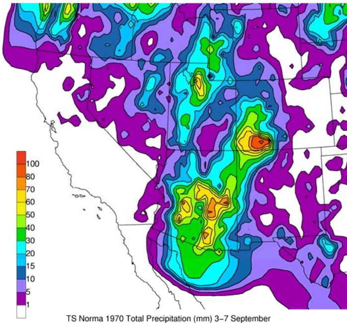
TS Norma 1970 Total Precipitation (mm) 3-7 September
