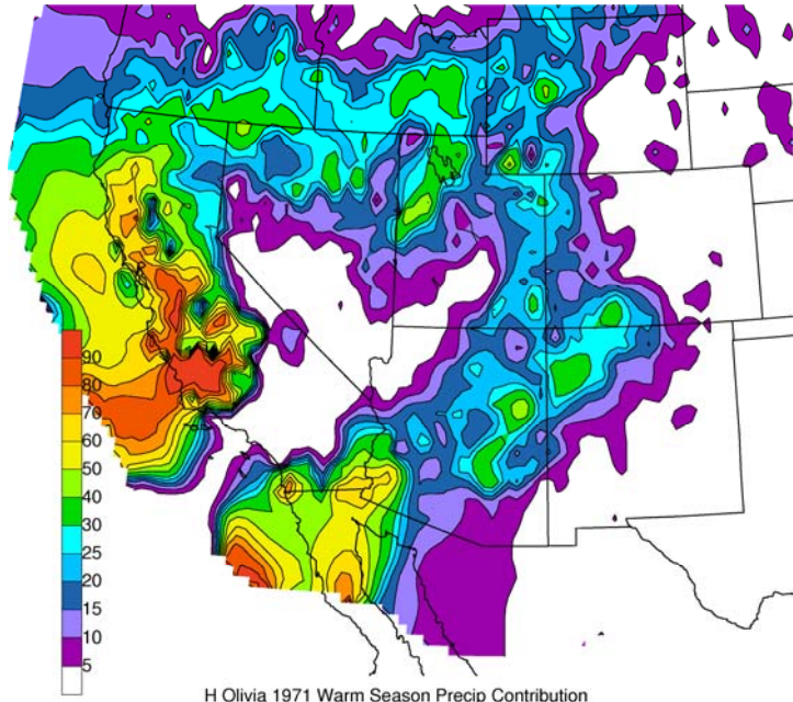
H Olivia 1971 Warm Season Precip Contribution
