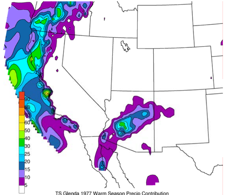
TS Glenda 1977 Warm Season Precip Contribution
