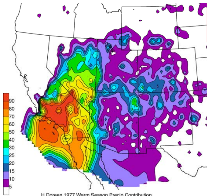
H Doreen 1977 Warm Season Precip Contribution
