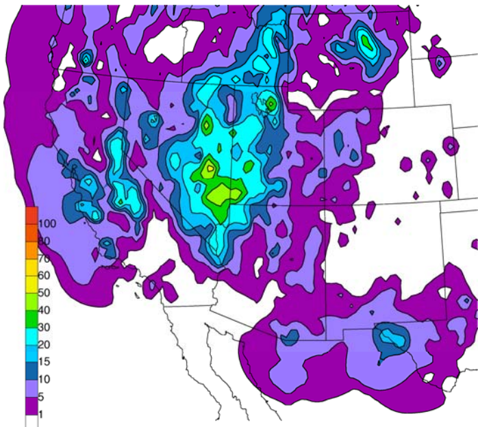
H Liza 1976 Total Precipitation (mm) 1-3 October
