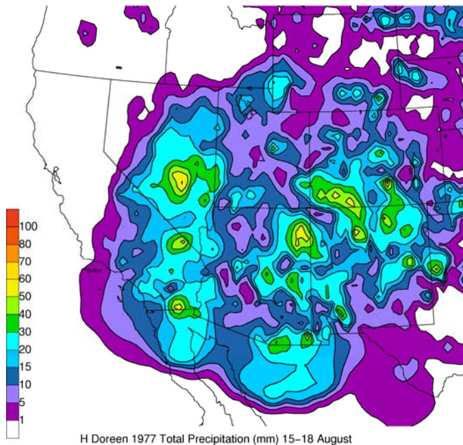
H Doreen 1977 Total Precipitation (mm) 15-18 August
