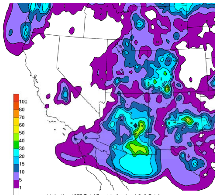
H Heather 1977 Total Precipitation (mm) 6-8 October
