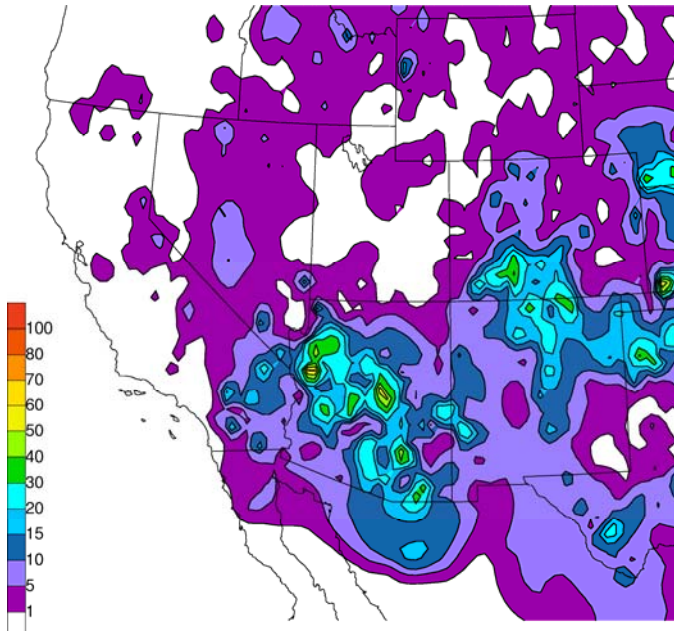
H Ignacio 2003 Total Precipitation (mm) 26-29 August
