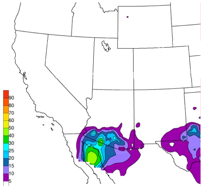
H Marty 1903 Warm Season Precip Contribution
