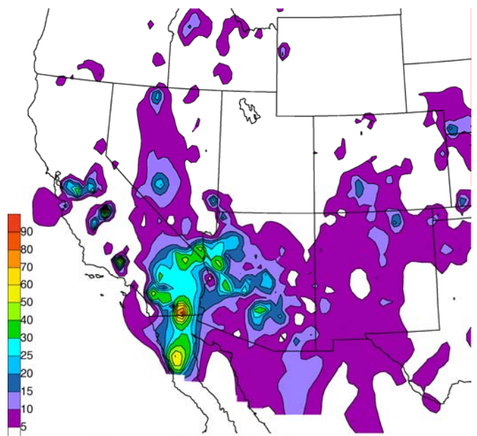
H Ignacio 1903 Warm Season Precip Contribution
