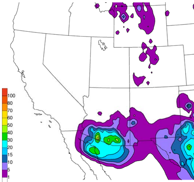
H Marty 2003 Total Precipitation (mm) 24-26 September
