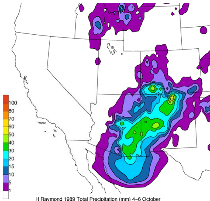
H Raymond 1989 Total Precipitation (mm) 4-6 October
