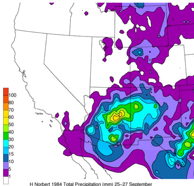
H Norbert 1984 Total Precipitation (mm) 25-27 September
