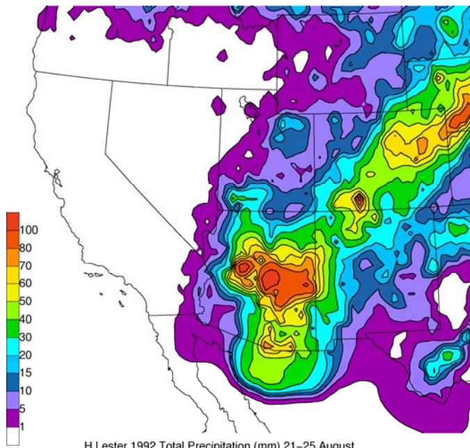
H Lester 1992 Total Precipitation (mm) 21-25 August
