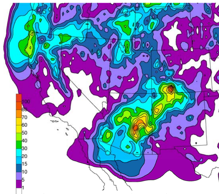
H Olivia 1971 Total Precipitation (mm) 29 September - 1 October
