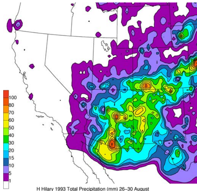
H Hilary 1993 Total Precipitation (mm) 26-30 August
