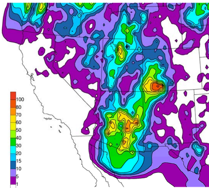
TS Norma 1970 Total Precipitation (mm) 3-7 September
