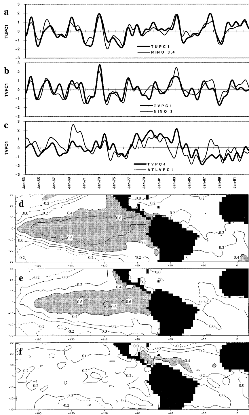
FIG. 9. (a) Score time series of T-UPC1 and Niño-3.4. (b) Score time series of T-VPC1 and Niño-3. (c) Score time series of T-VPC4 and ATLVPC1. All time series have been low-pass filtered, retaining frequencies <1 cycle \text{yr}^{-1} . All SST time series lead air temperature PCs by one month. (d) Same as Fig. 6a but for T-UPC1 (one-month lag). (e) Same as (d) but for T-VPC1 (one-month lag). (f) Same as (d) but for T-VPC4 (no lag).
