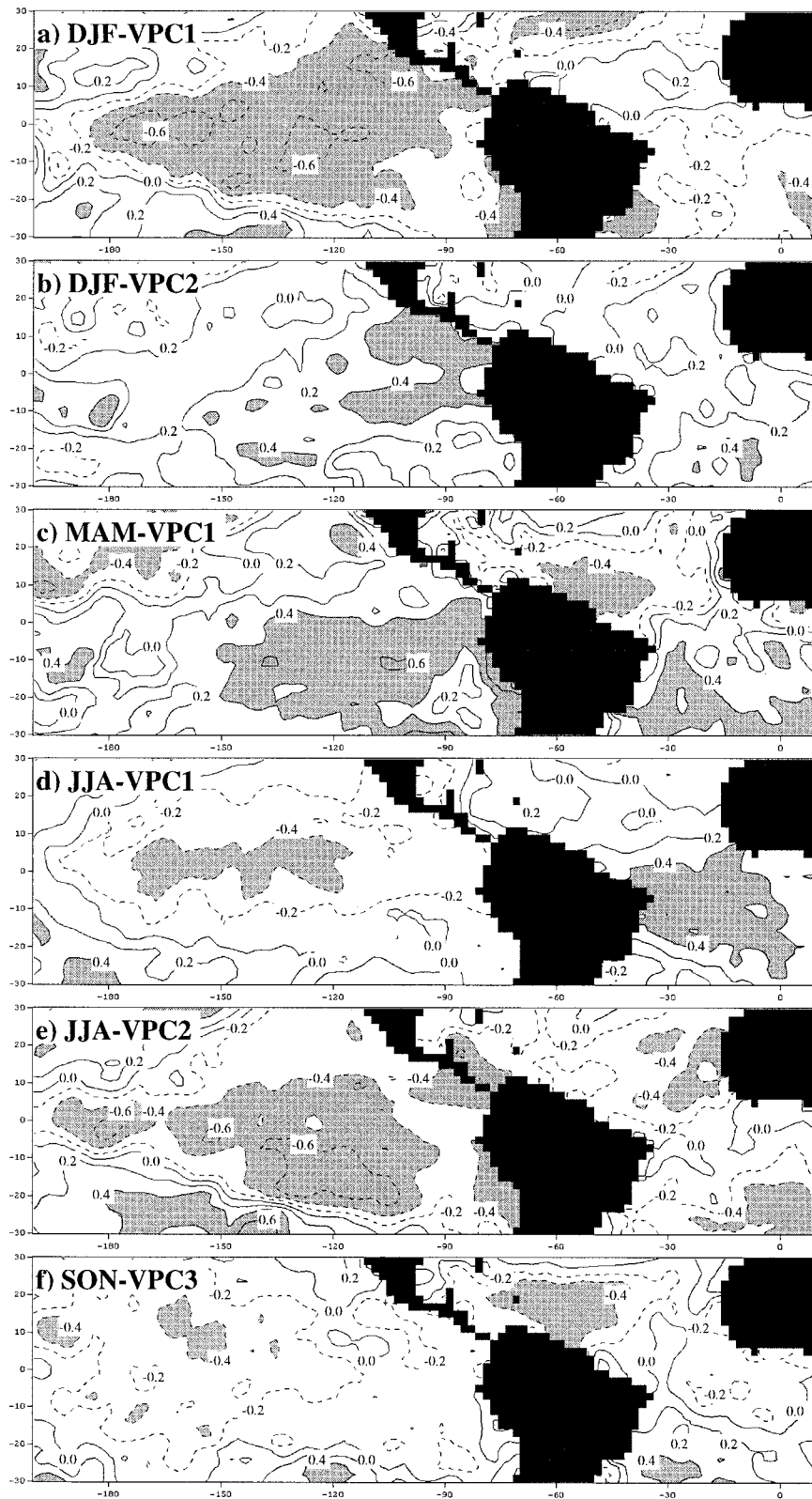
FIG. 6. (a) Pixel-based correlation of tropical Pacific and Atlantic SSTA in Dec with score time series of DJF-VPC1. Contour interval is 0.2; negative contours are dashed, and values < -0.4 and > 0.4 (significant at 95% level) are shaded. (b) Same as (a) but for DJF-VPC2. (c) Same as (a) but for MAM-VPC1 correlation with Mar SSTA. (d) Same as (a) but for JJA-VPC1 correlation with Jun SSTA. (e) Same as (d) but for JJA-VPC2. (f) Same as (a) but for SON-VPC3 correlation with Sep SSTA.
