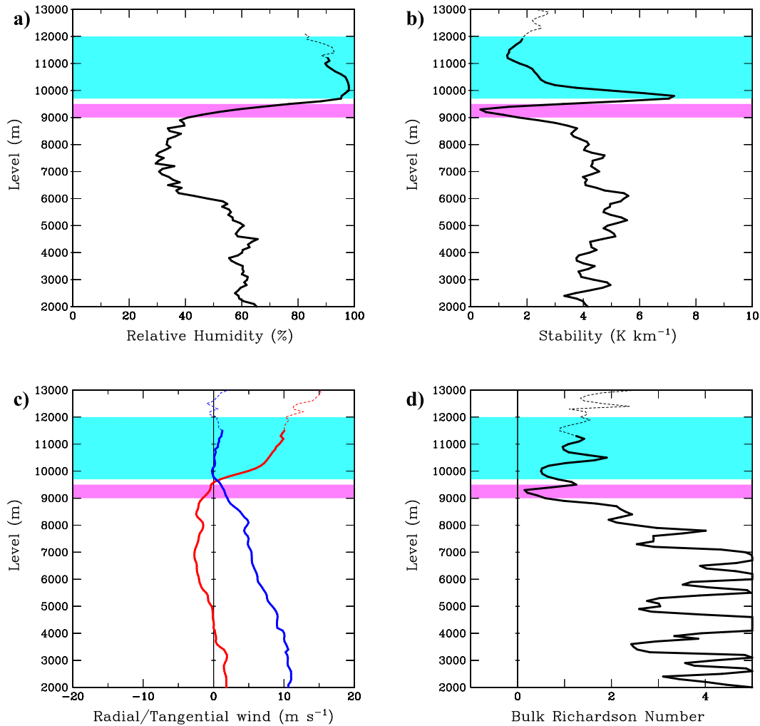
FIG. 8. Composite sounding for sondes that exhibited turbulent layers beneath cirrus cloud base. Composite is with respect to the turbulent layer shown by the magenta shading. Because the turbulent layer existed over a range of heights, the composites begin at 2 km. (a) Mean relative humidity with respect to ice ( T \leq 0^\circ\text{C} ) or water ( T > 0^\circ\text{C} ). The blue shading represents the cirrus layer. (b) Mean \partial\theta_v/\partial z ( \text{K km}^{-1} ). (c) Mean storm-relative radial velocity (red) and tangential velocity (blue; both \text{m s}^{-1} ). (d) R_B from Eq. (1) using the mean fields. Solid contours indicate levels where 10 or more values were available, dashed lines indicate 4–9 sondes, and no contour was plotted if fewer than 4 sonde observations were available.
