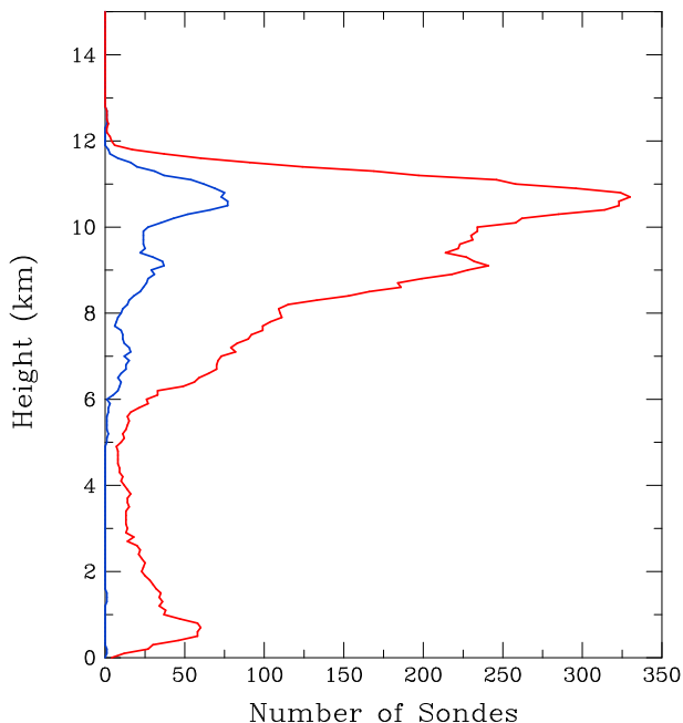
FIG. A1. Number of dropsondes that displayed saturation or supersaturation as a function of height. Blue indicates Hurricane Ivan (327 sondes); red indicates all G-IV data (2571 sondes).
