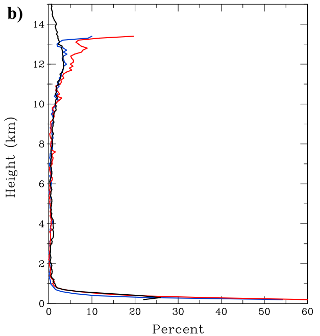
FIG. 3. (a) Percentage of sondes with R_B < 1 as a function of height. Black: non-tropical cyclone rawinsondes. Blue: G-IV sondes within 1000 km of tropical depressions, storms, and category-1 and -2 hurricanes. Red: G-IV sondes within 1000 km of major hurricanes. (b) As in (a), but for the percentage of R_B \leq 0.25 . Plotted points contain a minimum of 60 observations.
