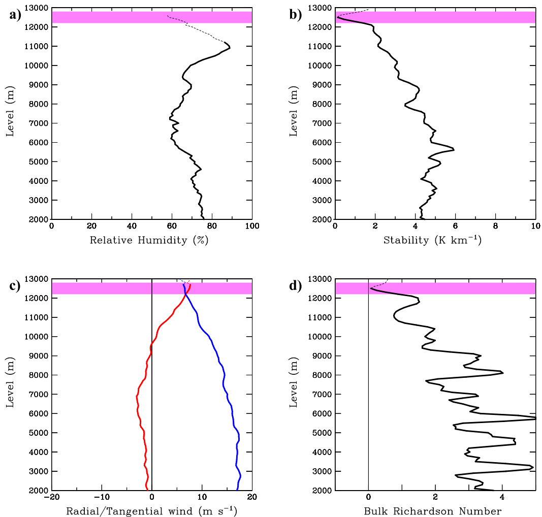
FIG. 11. As in Fig. 8, but for turbulent layers in the upper troposphere within the CDO produced by low stability in the absence of strong vertical wind shear. Solid contours indicate levels where 25 or more observations were available; dashed lines indicate 10–24 sondes. No contour was plotted if fewer than 10 sondes were available.
