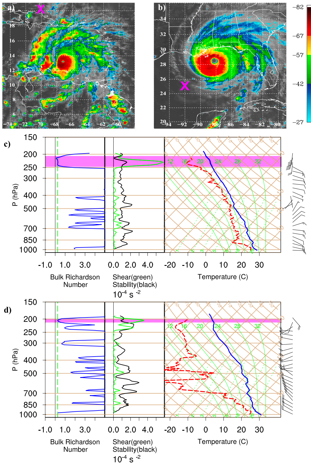
FIG. 12. As in Fig. 7, but for high-shear turbulent layers outside the CDO. These sondes were released at (a),(c) 1929 UTC 8 Sep and (b),(d) 2102 UTC 15 Sep.
