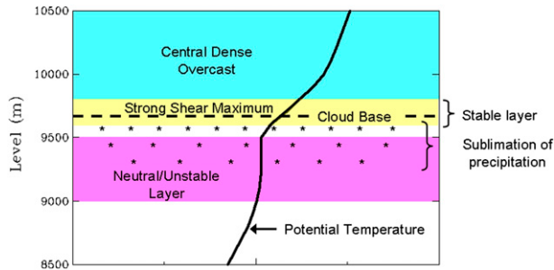
FIG. 9. Schematic diagram for turbulent layers beneath cloud base. The solid line represents the potential temperature from the beneath-cloud turbulence composite. Blue shading shows the cirrus layer, yellow shading shows the stable layer, and magenta shading shows the turbulent layer. The stars indicate sublimating snow or ice.
