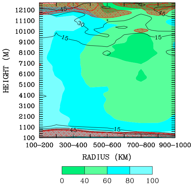
FIG. 6. Composite relative humidity with respect to ice ( T \leq 0^\circ\text{C} ) or water ( T > 0^\circ\text{C} ) for Hurricane Ivan (shaded). Black and red contours represent the percentage occurrence, respectively, of R_B < 1 (increment 15%) and R_B < 0.25 (stippled starting at 5%; increment 5%).
