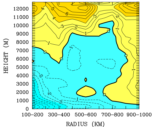
FIG. 5. Radius–height section of the mean storm-relative radial velocity (increment 1 \text{ m s}^{-1} ) for Hurricane Ivan (2004), in 100-km radial bins and 100-m vertical layers. Cyan represents inflow and yellow represents outflow. Darker cyan and yellow indicate radial components exceeding 4 \text{ m s}^{-1} .
