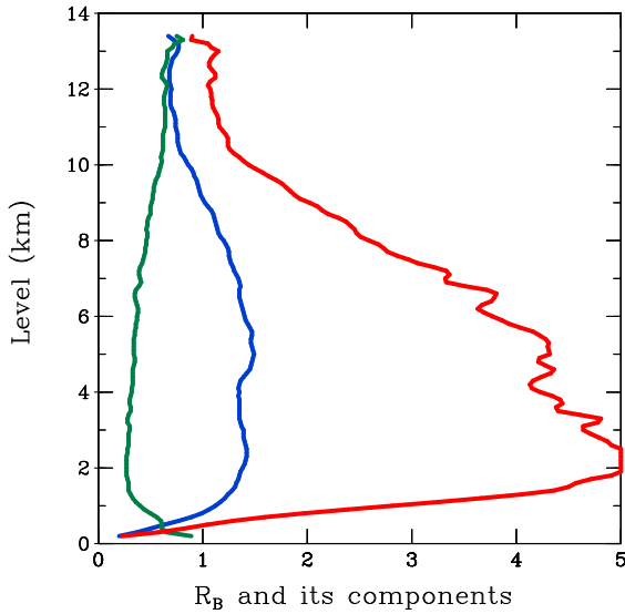
FIG. 2. Vertical profile of the numerator from Eq. (1) (stability term; blue), the denominator (shear-squared term; green), and the bulk Richardson number from these mean fields (red; values above 5 are set to 5). The R_B components have units of 10^{-4} \text{ s}^{-2} . These calculations include all G-IV sondes.
