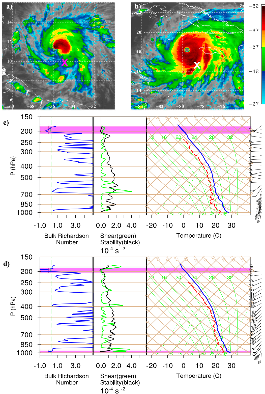
FIG. 10. As in Fig. 7, but for turbulent layers in the upper troposphere produced by low stability in the absence of strong vertical wind shear. These sondes were released at (a),(c) 2227 UTC 6 Sep and (b),(d) 2310 UTC 11 Sep.
