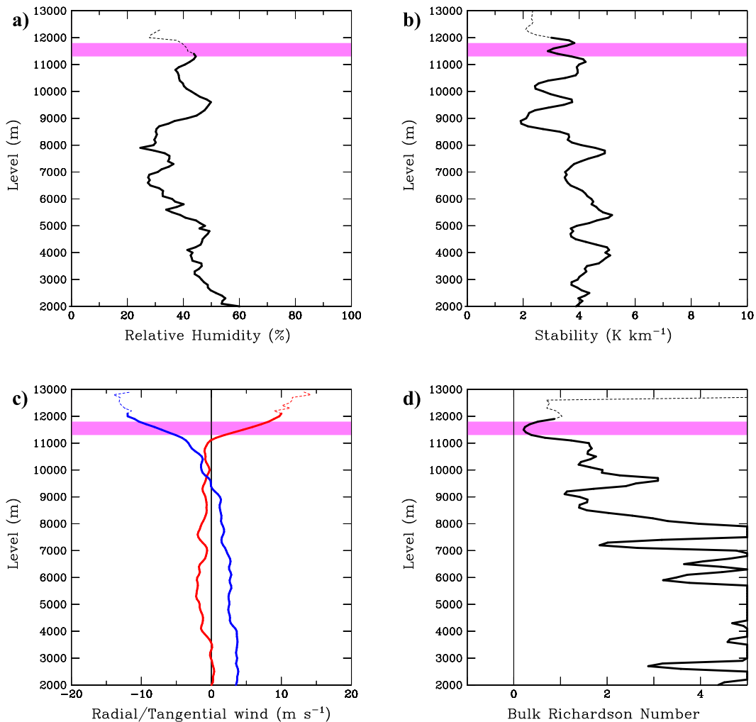
FIG. 13. As in Fig. 8, but for high-shear turbulent layers outside the CDO. Solid lines indicate levels where 10 or more observations were available; dashed lines indicate 4–9 observations.
