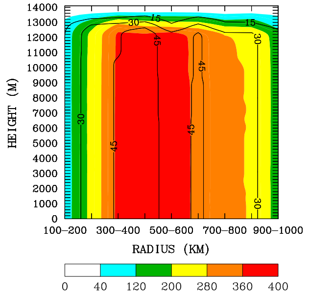
FIG. 1. Number of sondes used in this study within 100-km radial bins and 100-m vertical layers. Color shading: total number of G-IV sondes. Contours: number of G-IV sondes in Hurricane Ivan alone.
