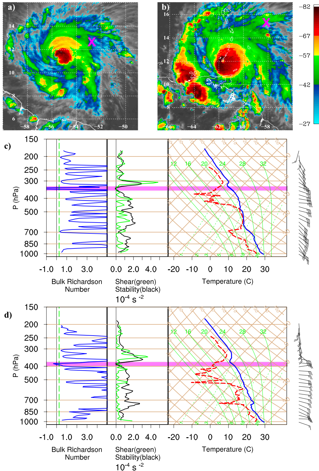
FIG. 7. Two examples of turbulent layers beneath cirrus cloud base within the CDO of Hurricane Ivan. (top) Infrared satellite images at the time closest to the sonde release (crosses show the release locations): (a) 2156 UTC 6 Sep and (b) 2026 UTC 7 Sep. (c),(d) Vertical profiles for the sondes in (a),(b), respectively: (left) bulk Richardson number, (middle) vertical profiles of the stability term (black) and the shear-squared term (green) from Eq. (1) (units for both are 10^{-4} \text{ s}^{-2} ), and (right) skew T - \log p diagrams for each sonde (solid blue shows temperature and dashed red shows dewpoint). Each long wind barb is 5 \text{ m s}^{-1} and each short barb is 2.5 \text{ m s}^{-1} . The magenta band shows the turbulent layer.
