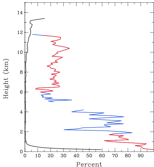
FIG. A2. Black indicates percentage of G-IV sondes that met the dry turbulence criterion using Eq. (1) (equivalent to the sum of the blue and red curves in Fig. 3b). Red indicates percentage of sondes in saturated layers that met the moist turbulence criterion [using Eq. (A1) to estimate the Brunt–Väisälä frequency] when at least 26 sondes (1% of the total) were available. Blue is similar to red, but indicates when at least 10 sondes were available. Missing contour indicates fewer than 10 observations.
