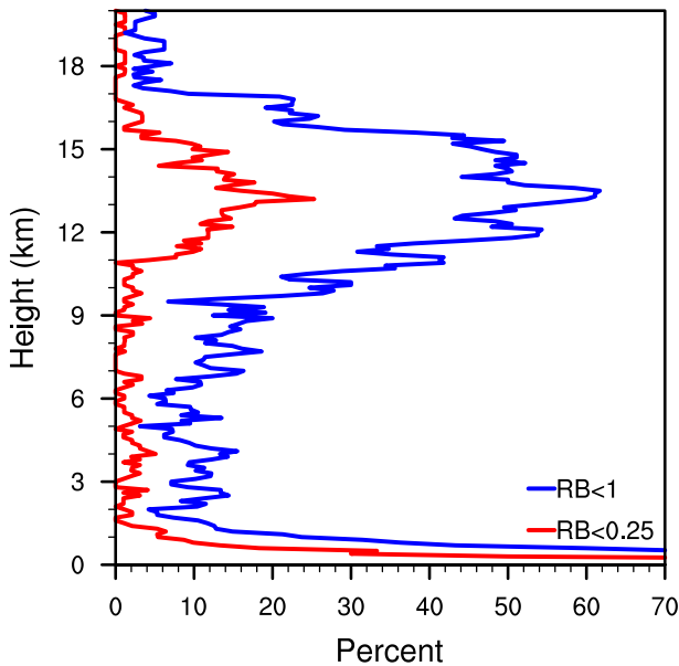
FIG. 4. Percentage of rawinsondes having R_B < 1 (blue) and R_B < 0.25 (red), calculated from the surface to the 20-km elevation from all rawinsondes within 500 km of a major hurricane.
