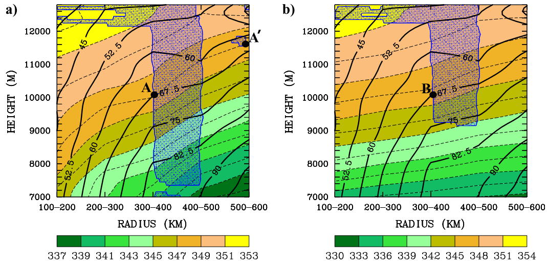
FIG. 5. (a) Mean absolute angular momentum, as in Fig. 4, plotted with \theta_e (shaded with dashed lines; increment: 1 K). (b) As in (a), but with \theta_v replacing \theta_e . Blue stippling represents regions of (a) moist and (b) dry symmetric instability. Points A, A', and B are discussed in the text.
