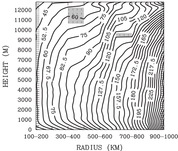
FIG. 2. Radial-vertical cross section of mean absolute angular momentum from Eq. (1) (increment: 7.5 \times 10^5 \text{ m}^2 \text{ s}^{-1} ) in 100-km radial and 100-m vertical resolutions. Stippling indicates the region where M decreased outward.
