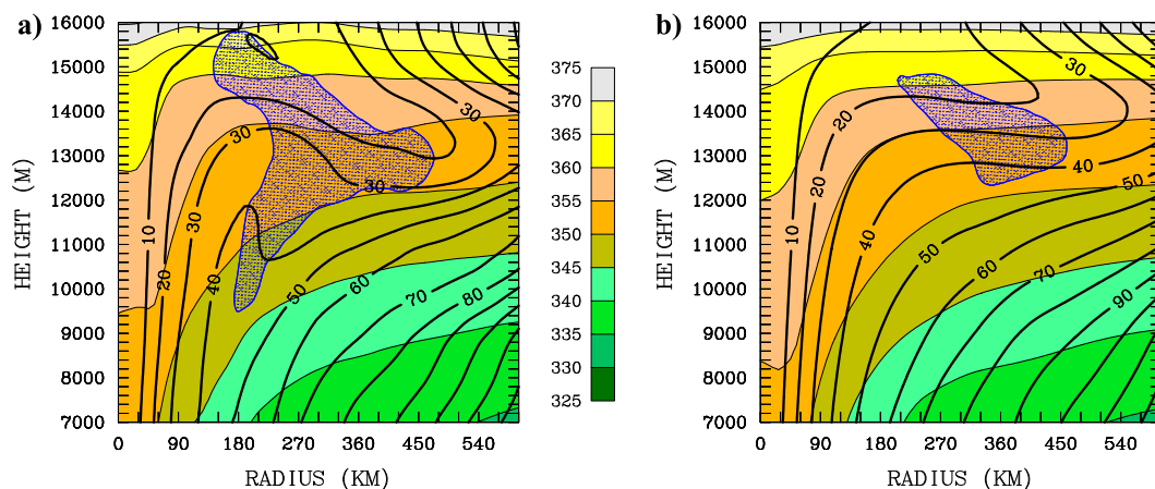
FIG. 6. (a) Azimuthally averaged absolute angular momentum (dark black contours; increment: 10 \times 10^5 \text{ m}^2 \text{ s}^{-1} ) and equivalent potential temperature (shaded) from the hurricane nature run of Nolan et al. (2013), valid at 1500 UTC 3 Aug. The blue stippling indicates the region of inertial instability, which is nearly identical to that for moist symmetric instability. (b) As in (a), but for a 48-h mean beginning 0000 UTC 3 Aug.
