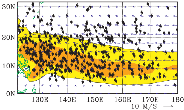
FIG. 3. As in Fig. 1, but the long-term mean 850-hPa relative vorticity and wind are averaged from July to November, and all July–November tropical cyclone formation locations are shown.
