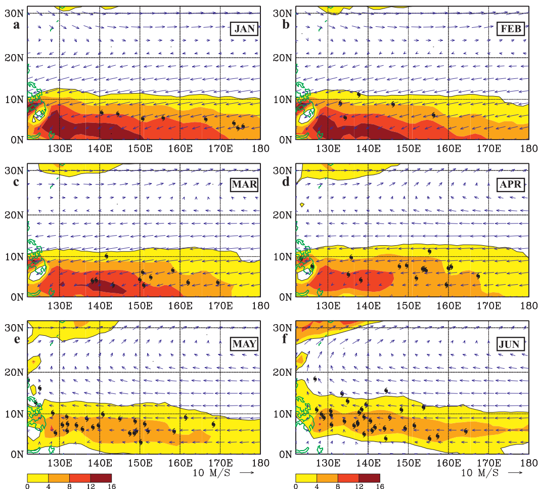
FIG. 1. Long-term mean (1988–2010) northwest Pacific 850-hPa relative vorticity ( 10^{-6} \text{ s}^{-1} ; shaded for positive values only) and mean 850-hPa winds (vectors). Formation locations for tropical cyclones (symbols) for each month are obtained from the Joint Typhoon Warning Center: (a)–(f) January–June and (g)–(l) July–December.
