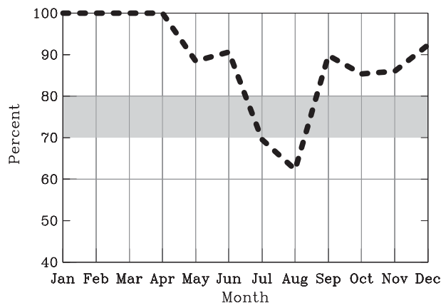
FIG. 2. Percentage of tropical cyclones forming within the long-term monthly mean MT positions shown in Fig. 1. The shading represents 70%–80%.
