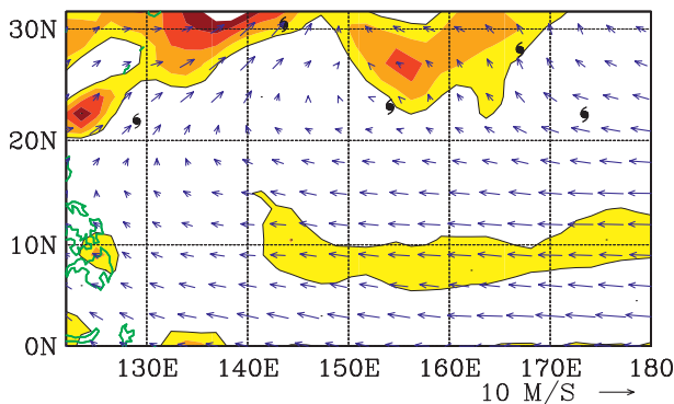
FIG. 5. As in Fig. 1, but for the single month of August 1988.
