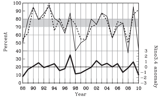
FIG. 4. Percentage of tropical cyclones forming each year within the climatological July–November mean MT shown in Fig. 3 (dashed line) and the July–November mean positive \zeta_{850} region for the same year (top solid line). Niño-3.4 index averaged July–November each year (bold solid line). Shading as in Fig. 2.
