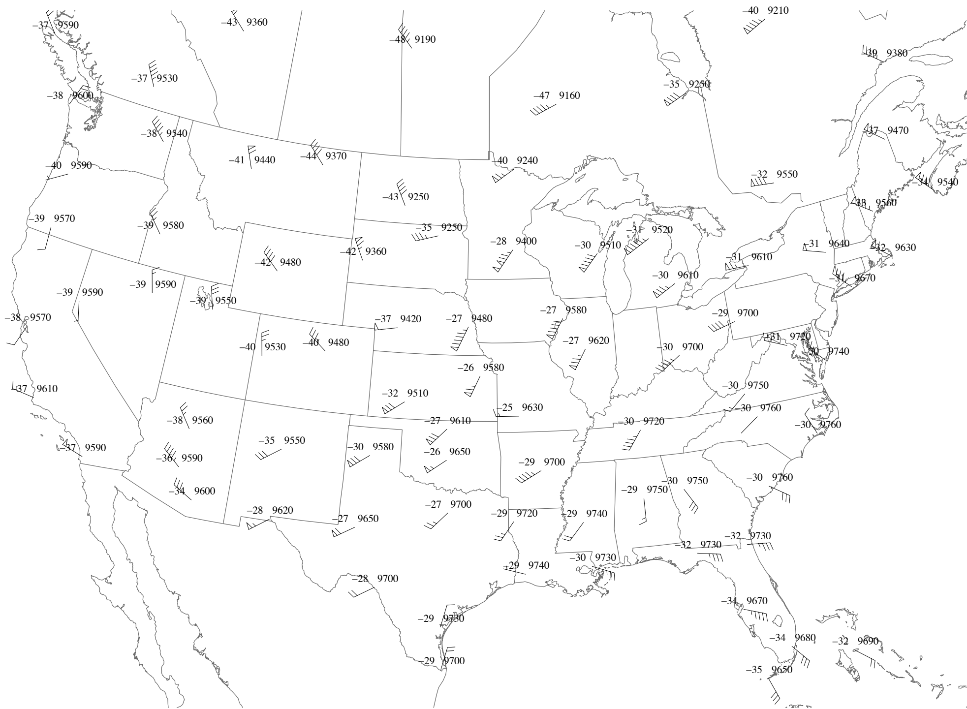
080914/1200 300-mb Observations
