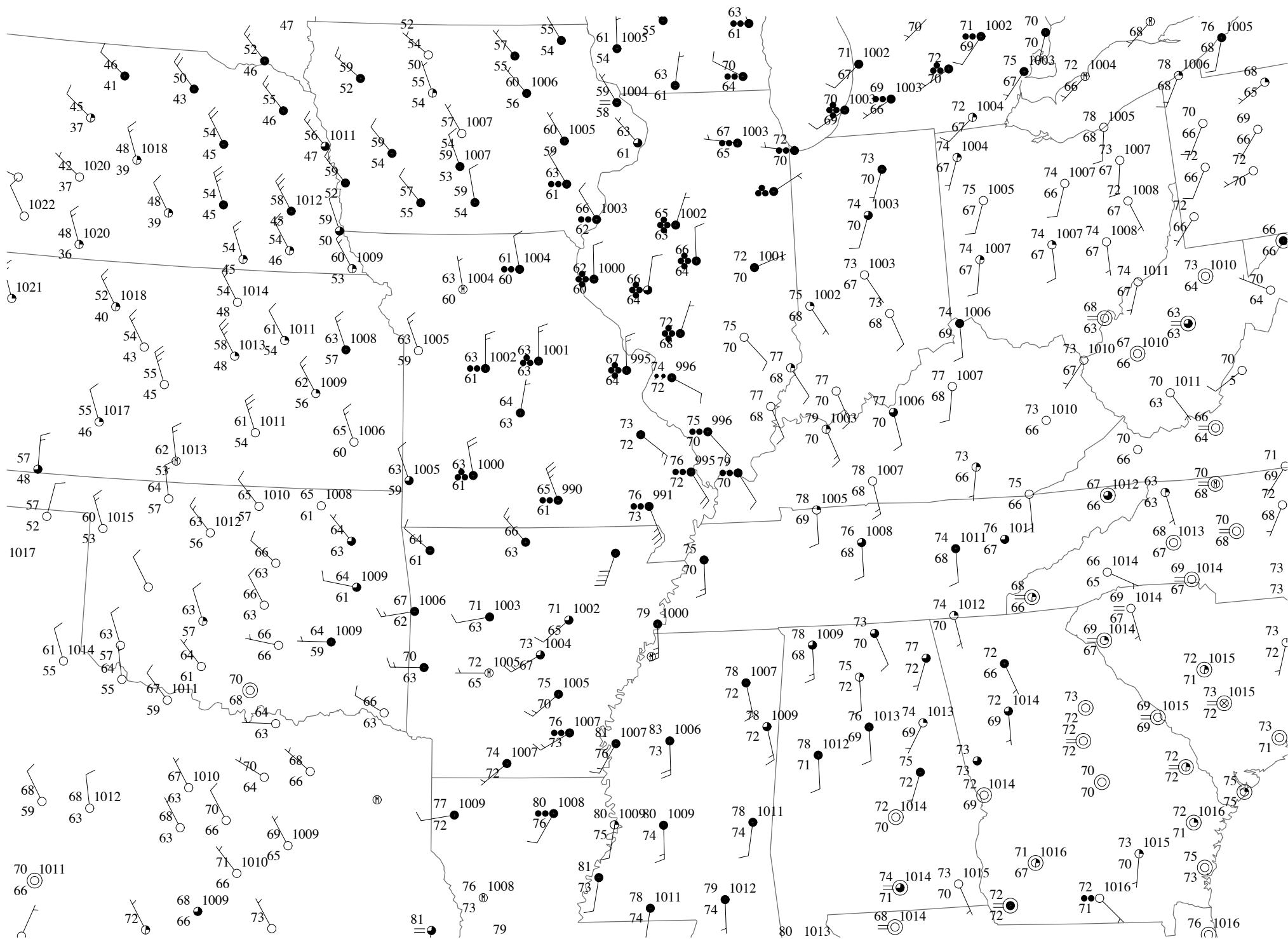
080914/1100 Surface Observations
