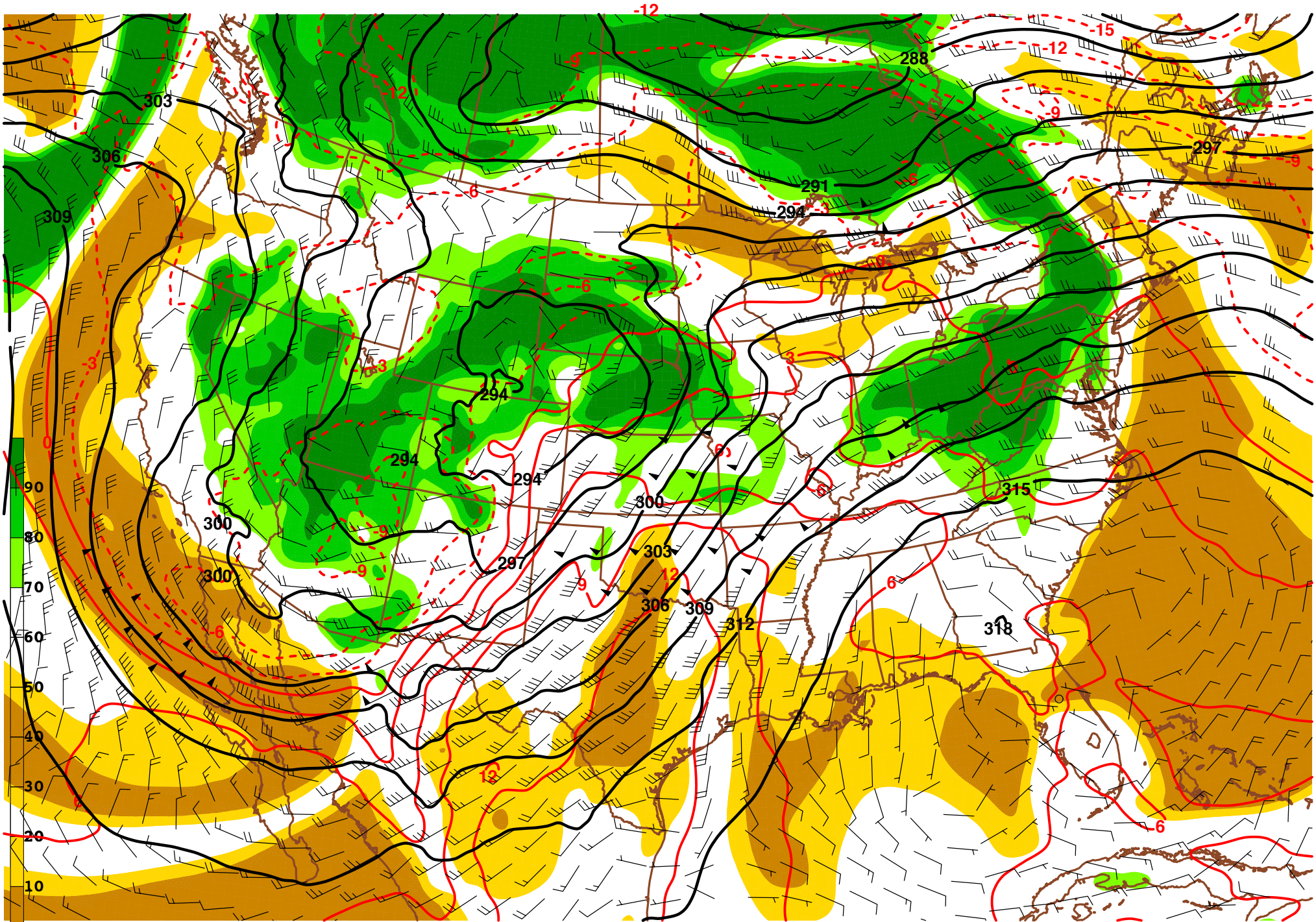
00Z Day 2 - 700-mb RH, Temp (C), Height (dam), and Wind (kt.)
