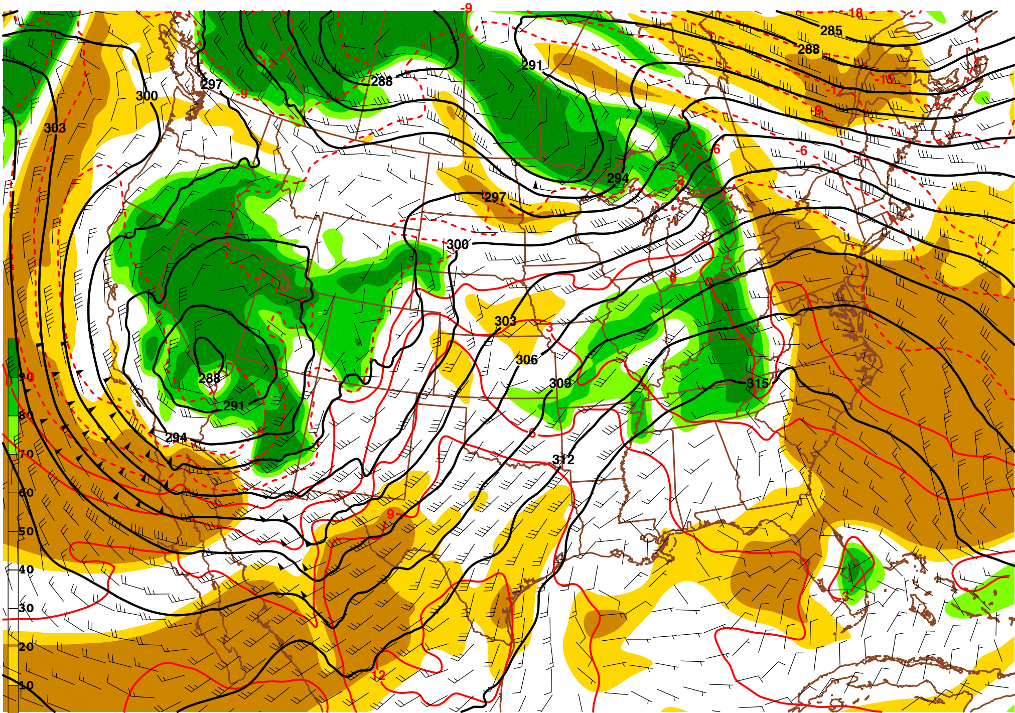
12Z Day 1 - 700-mb RH, Temp (C), Height (dam), and Wind (kt.)
