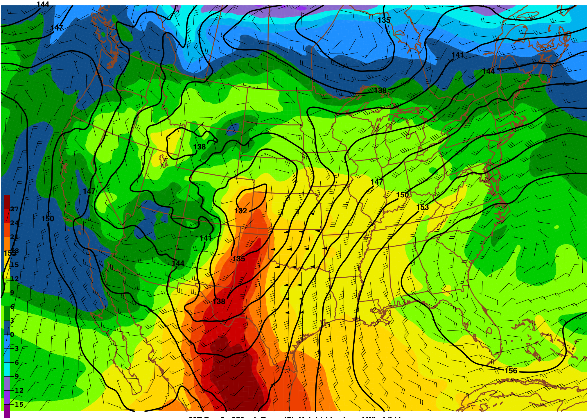
00Z Day 2 - 850-mb Temp (C), Height (dam), and Wind (kt.)
