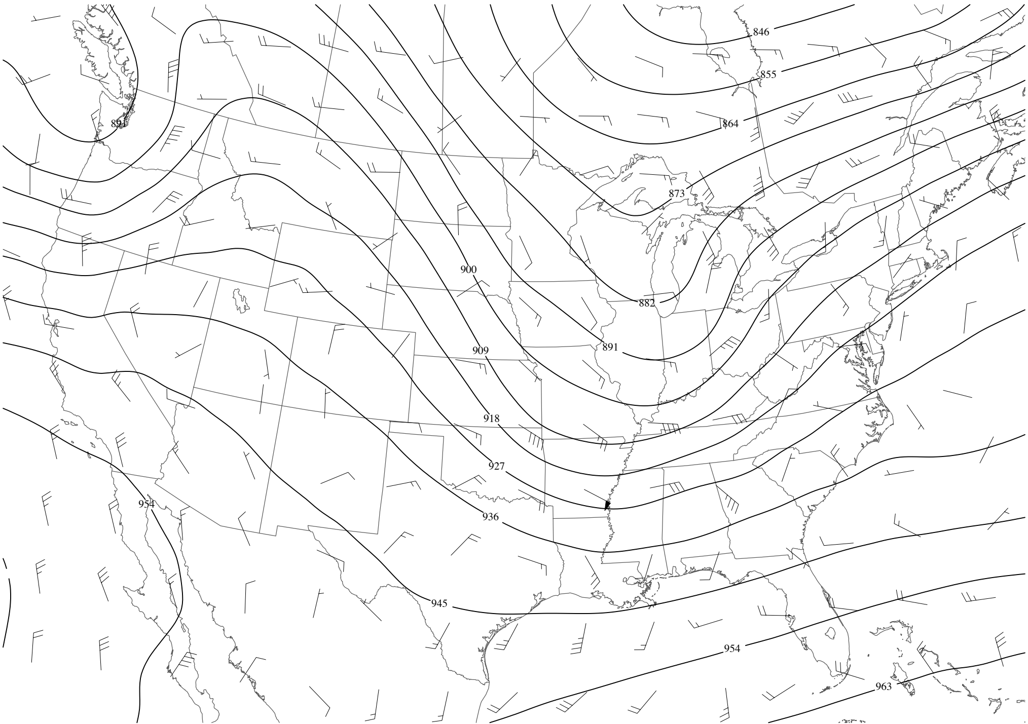
160302/0000F000 300-mb Height and Ageostrophic Wind ... MAP 2
