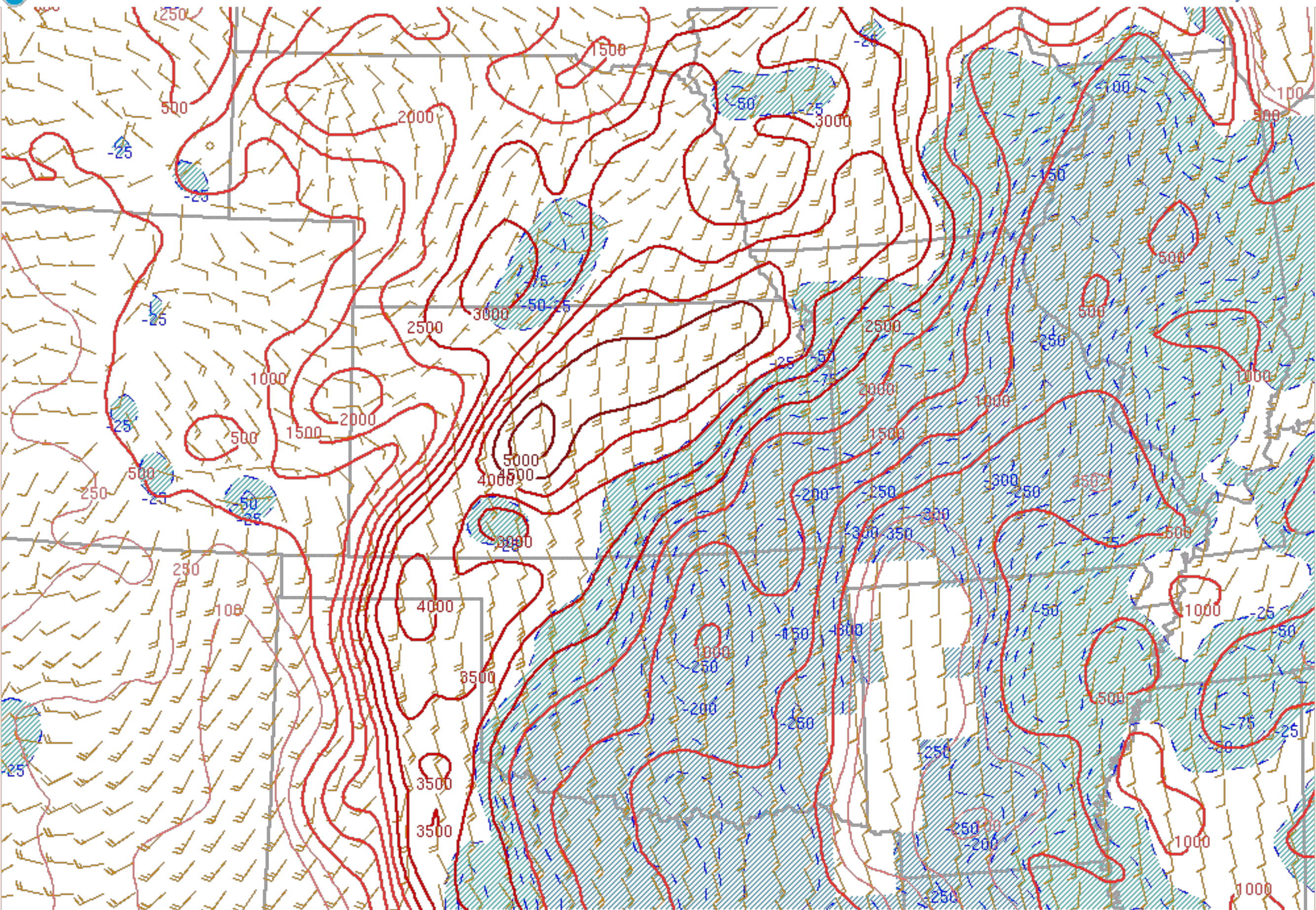
170516/2000 SBCAPE (contour) and SBCIN (J/kg, shaded)
