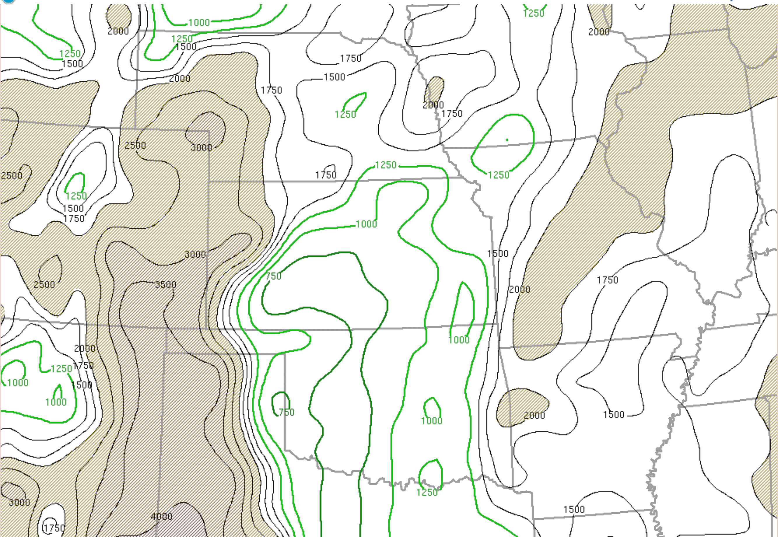
170516/2200 100 mb mean parcel LCL height (m AGL)
