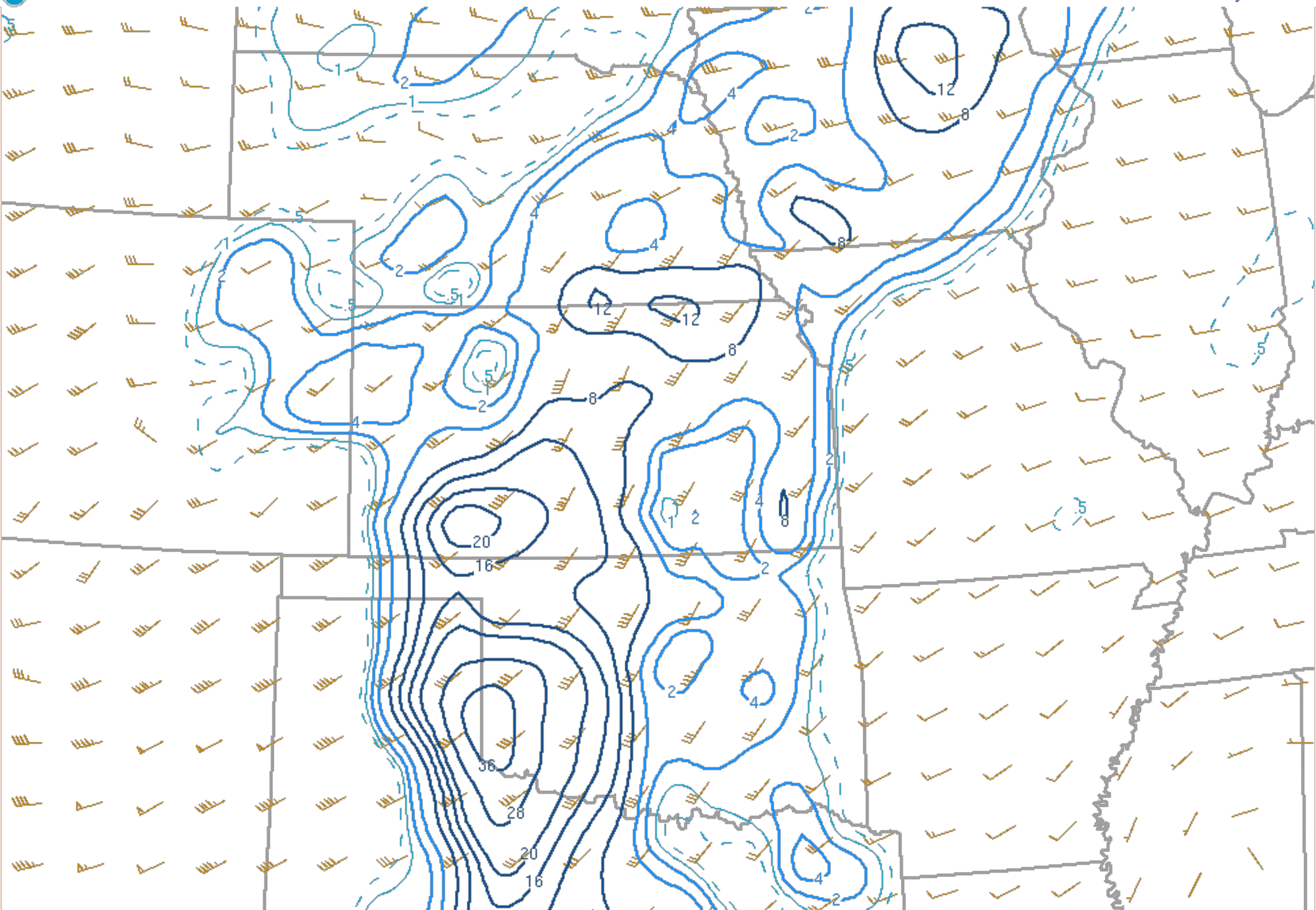
170517/0000 Supercell Composite Parameter (eff layer) and Bunkers storm motion (kt)
