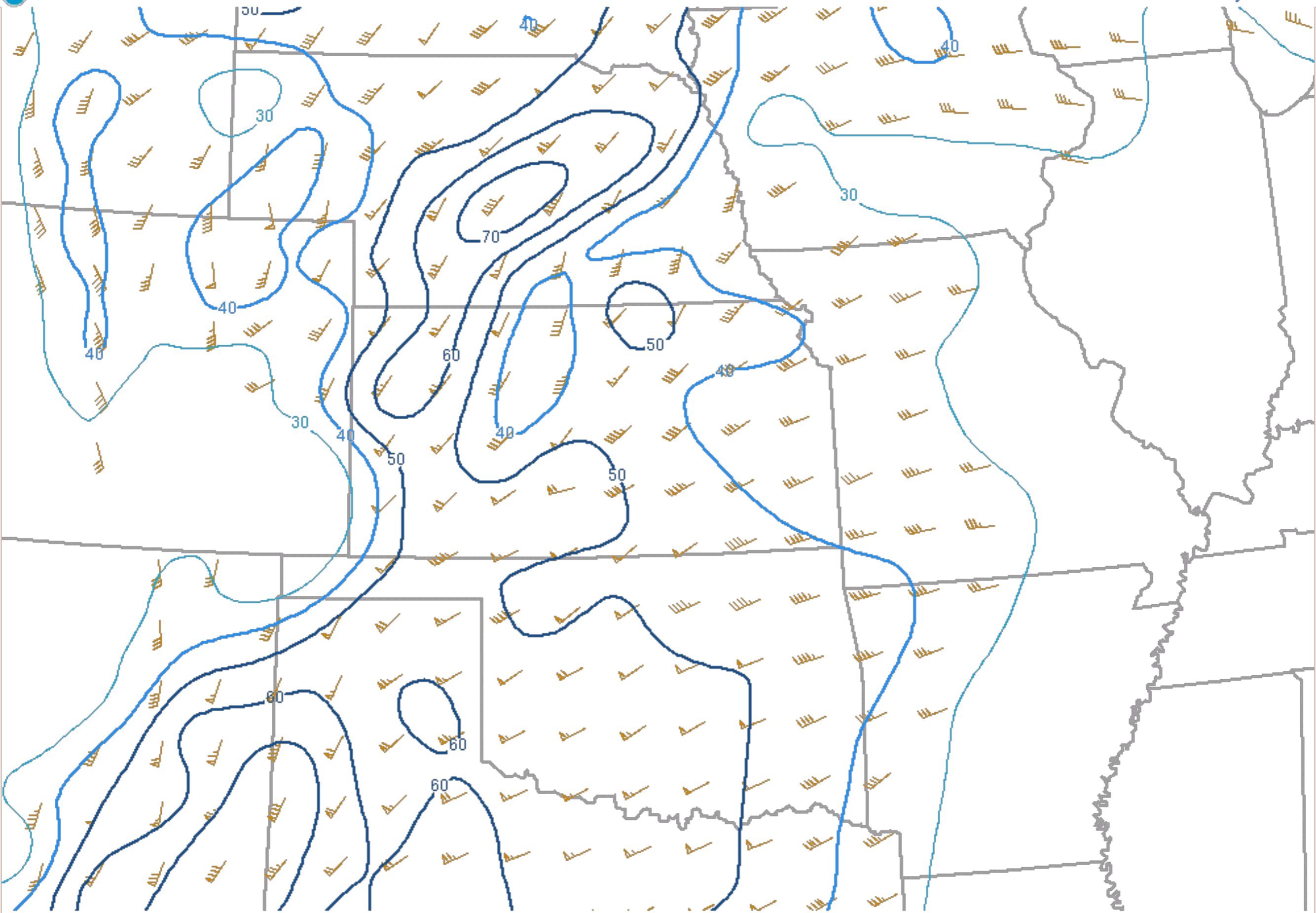
170517/0000 Surface to 6 km shear vector (kt)
