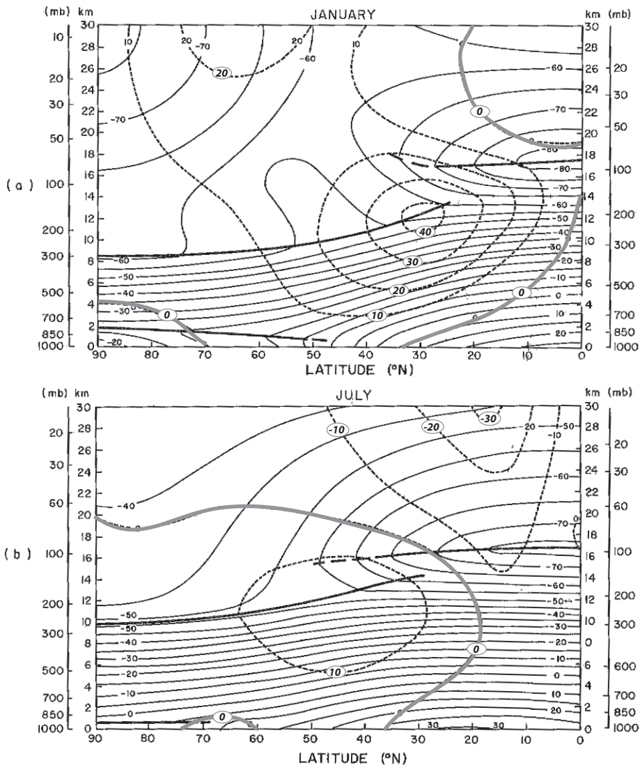
Fig. 1.11 Meridional cross sections of longitudinally averaged temperature in degrees Celsius (—) and zonal wind in meters per second (---) for the northern hemisphere in January (a) and July (b). Positive zonal winds indicate flow from west to east. Heavy lines denote the tropopause and the Arctic inversion. (After Arctic Forecast Guide , U.S. Navy Weather Research Facility, 1962.)
