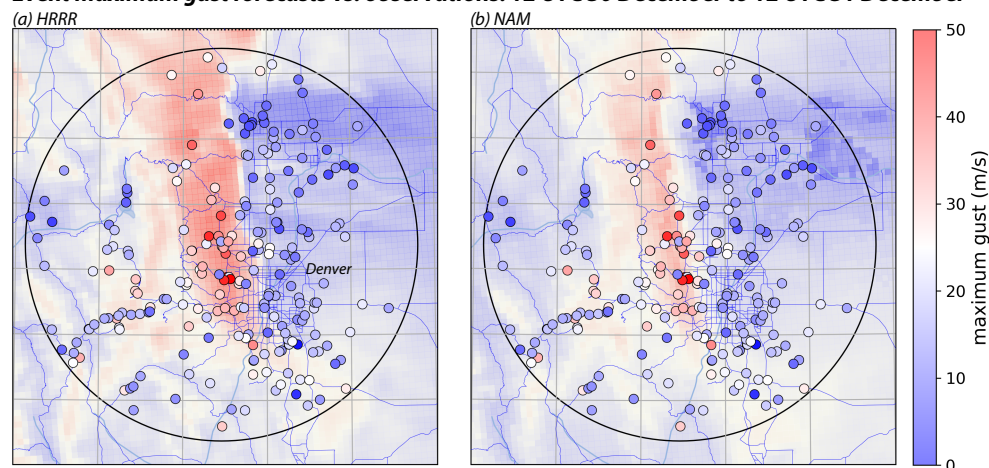
Figure 13. Event maximum gust forecasts (shaded, m/s) from the 1200 UTC 30 December 2021 (a) HRRR and (b) NAM cycles, compared to observed gust maxima for stations within 100 km of Boulder (indicated by the black circle). Comparison limited to a 24 h period spanning the windstorm. See text for filtering employed for observations.
