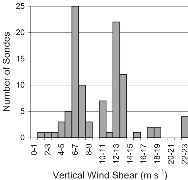
FIG. 2. Number of dropsondes in each 1 \text{ m s}^{-1} range of ambient vertical wind shear.
