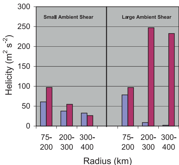
FIG. 4. Radial variation of 0–3-km helicity ( \text{m}^2 \text{ s}^{-2} ) averaged over 75–200, 200–300, and 300–400 km for TCs experiencing (left) small and (right) large ambient shear. Upshear means are in blue and downshear in red.
