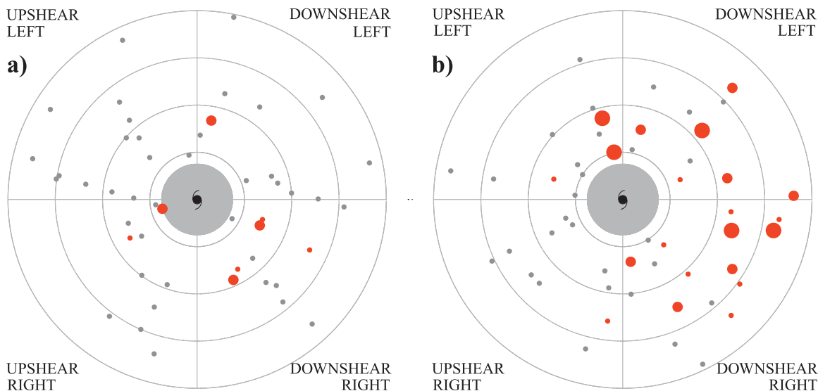
FIG. 3. Location of dropsondes and 0–3-km helicity values for (a) small ambient vertical wind shear and (b) large ambient shear. Dropsonde locations have been positioned with respect to the moving center at the time of their splashdown and have been rotated with respect to the ambient vertical wind shear following Corbosiero and Molinari (2002). The right half represents downshear. Range circles are shown every 100 km. Gray dots represent helicity <100 \text{ m}^2 \text{ s}^{-2} ; small red dots 100 \text{ m}^2 \text{ s}^{-2} \leq \text{SREH} < 200 \text{ m}^2 \text{ s}^{-2} ; medium red dots 200 \text{ m}^2 \text{ s}^{-2} \leq \text{SREH} < 300 \text{ m}^2 \text{ s}^{-2} ; large red dots \geq 300 \text{ m}^2 \text{ s}^{-2} . Helicity was not calculated within 75 km of the center (shaded) because of potential errors associated with sonde drift.
