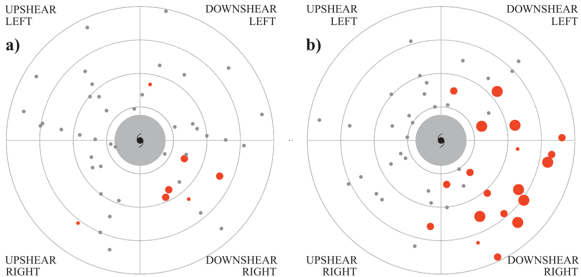
FIG. 7. As in Fig. 3, but showing EHI, for TCs experiencing (a) small and (b) large ambient shear. Gray dots represent EHI < 0.6 ; small red dots 0.6 \leq EHI < 1.0 ; medium red dots 1.0 \leq EHI < 2.0 ; large red dots EHI \geq 2 .
