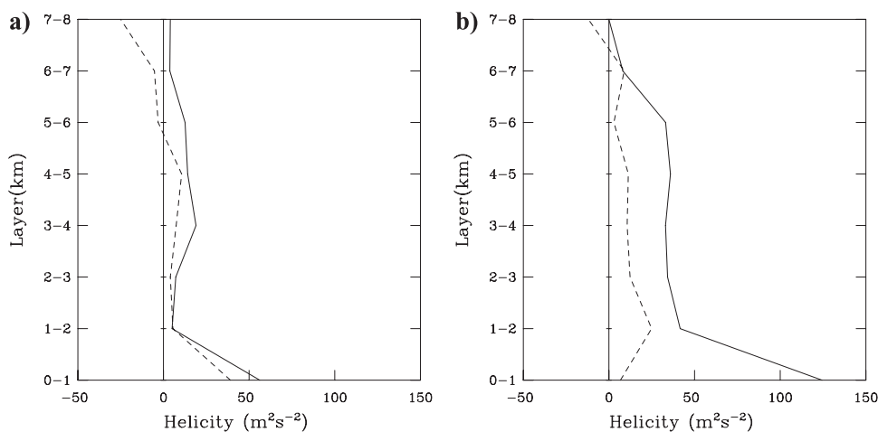
FIG. 6. Vertical profile of helicity ( \text{m}^2 \text{ s}^{-2} ) in 1-km layers, averaged over upshear (dashed) and downshear (solid) soundings, for TCs experiencing (a) small and (b) large ambient wind shear.
