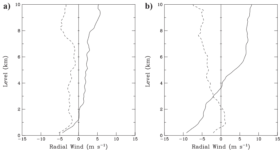
FIG. 5. Mean radial velocity ( \text{m s}^{-1} ) for downshear (solid) and upshear sondes (dashed) for TCs experiencing (a) small and (b) large ambient vertical wind shear. The z = 0 and z = 100\text{-m} levels are not shown because of insufficient observations.
