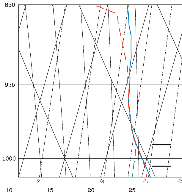
FIG. 1. Example of the Bogner et al. (2000) correction for erroneous boundary layer moisture for a sounding taken in Hurricane Erin (2001). Shown are temperature (blue solid), dewpoint (red dashed), and modified dewpoint (green dashed). The bracketed layer meets the criteria for the correction: relative humidity >98\% and lapse rate >8 \text{ K km}^{-1} .
