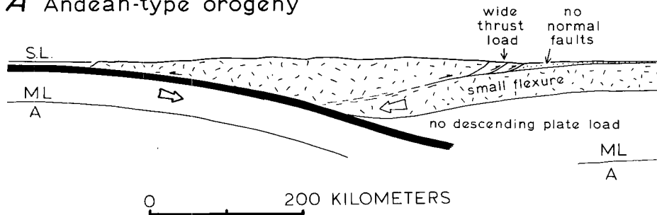
Figure 14. Generalized cross sections comparing Andean-type foreland basins, where the angle of flexure in the outer slope of the foreland basin is too gentle to cause normal faulting, and arc-continent collision settings, where the flexure is larger and normal faulting occurs.
