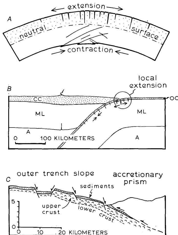
Figure 1. (A) Extensional deformation in the convex outer arc of this experimentally deformed material is accommodated by the opening of dilatant cracks that die out downward toward a neutral surface (from Ramsay, 1967, p. 401; no scale shown in original diagram). (B) Schematic representation of crustal-scale tension gashes formed as a result of lithospheric flexure at a subduction zone, adapted from an illustration by Isacks and others (1968). Arrows show opening and closing of dilatant cracks as the plate bends, then unbends. A is asthenosphere; ML is mantle lithosphere; OC is oceanic crust; CC is continental crust. (C) Typical representation of a normal faulted outer trench slope showing horst and graben topography and downward disappearance of normal faults (from Karig and Sharman, 1975).
