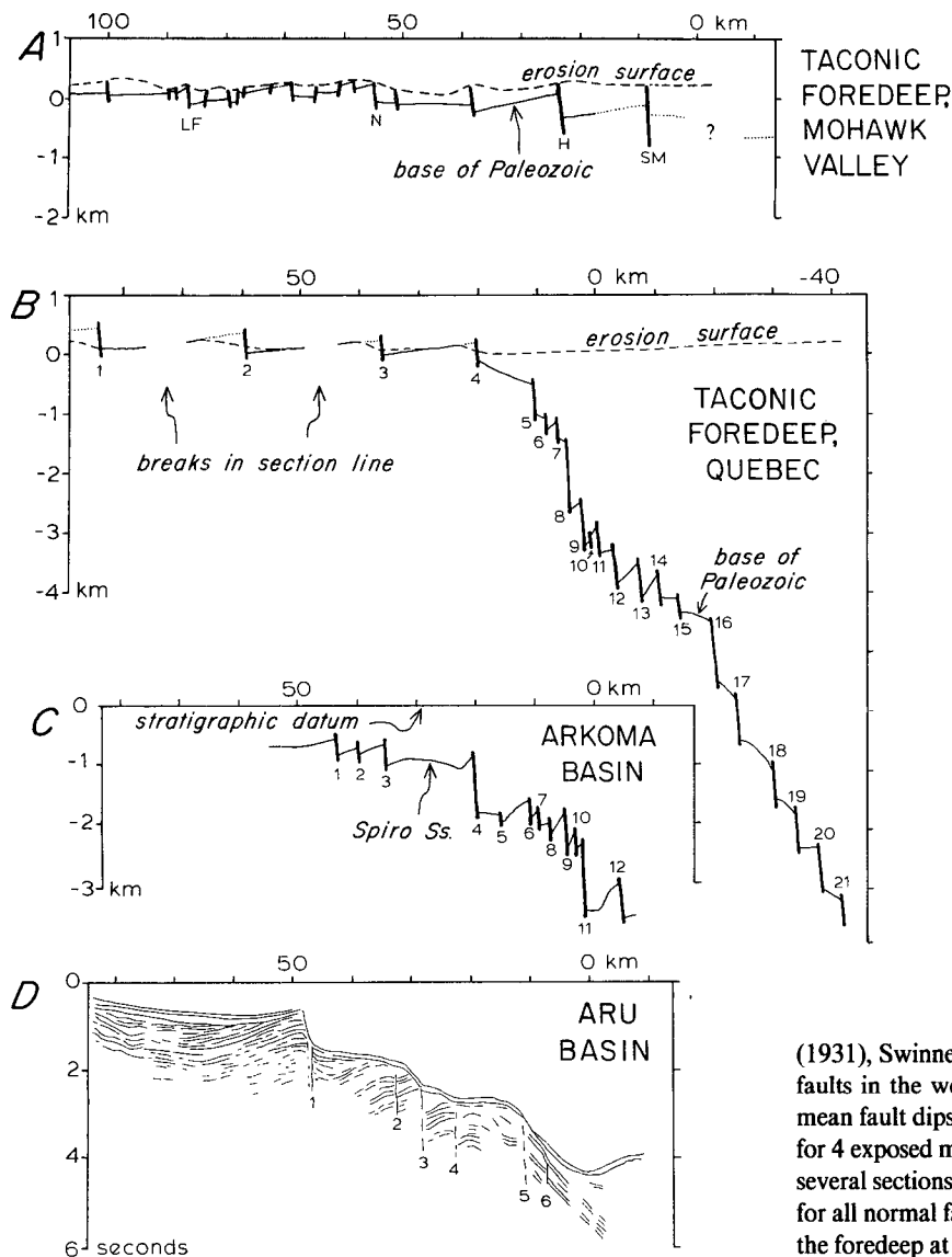
Figure 11. Comparative profiles across normal faulted foredeeps. The profiles are drawn at the same vertically exaggerated scales and are aligned horizontally with 0 km at the thrust front. (A) Taconic foredeep, Mohawk Valley, New York, based on this study. Datum is present-day horizontal, and the offset marker (thin line, dotted where approximate) is the Proterozoic-Paleozoic contact; it is cut by faults shown as thicker lines. Dashed line is the present erosion surface (B) Taconic foredeep, Quebec, including the cross section in Figure 10a, plus four additional faults closer to the craton (see Fig. 2). (C) Arkoma Basin, Arkansas, adapted from Houseknecht (1986). Datum is a key bed in the Atoka Formation, and the offset marker is the basal Atokan Spiro Sandstone. (D) Aru Basin, Australia-Banda Arc collision zone (section A-A' in Figure 12b, redrawn from a seismic reflection profile illustrated in Jacobson and others (1979), at approximately the same vertical scale (1.5 sec equals 1 km) as the other profiles. In each profile, note the stepwise descent of the underthrust plate beneath the orogenic belt.
