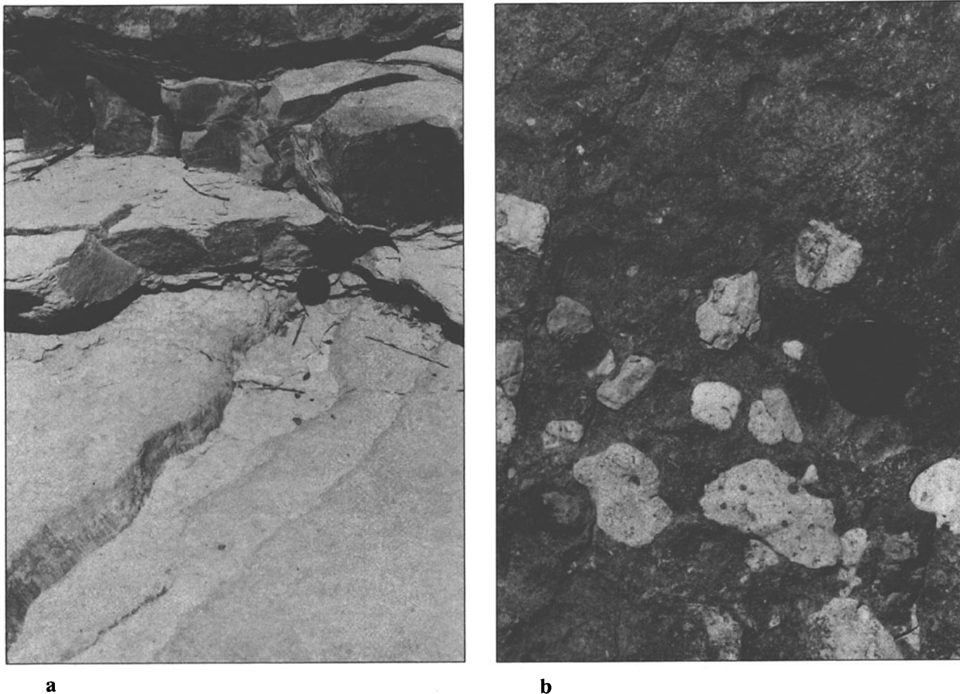
Figure 8. (a) View toward the north-northeast of minor synthetic (right-dipping) and antithetic normal faults cutting Black River Group carbonates at Inghams Mills. Slickensides plunge down the dip of fault planes. Lens cap for scale. (b) Limestone-matrix conglomerates in the Trenton Group at Inghams Mills (Fig. 3), between the Dolgeville and Manheim faults. The conglomerates, which contain clasts of subjacent Cambrian and Ordovician carbonates and Proterozoic basement gneisses, are inferred to have been shed from a nearby fault scarp, probably the Little Falls fault.
