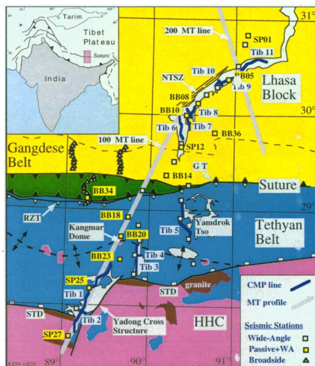
Fig. 1. Generalized geologic map of the INDEPTH transect region showing locations of INDEPTH controlled-source seismic, earthquake, and magnetotelluric recording programs. "CMP line," near-vertical incidence common midpoint reflection profile. "MT profile," approximate line of magnetotelluric recording stations; "Seismic stations," temporary seismic stations (REFTEKs) established for wide-angle recording of CMP shots ("Wide-Angle" and "Broadside") and broadband earthquake recording ("Passive"). The geologic base map is generalized from published sources (20, 43) and local geological observations made by INDEPTH personnel. HHC, High Himalayan crystallines; STD, South Tibetan detachment system; RZT, Renbu-Zedong thrust; GT, Gangdese thrust; NTSZ, Nyainqentanghla shear zone.
