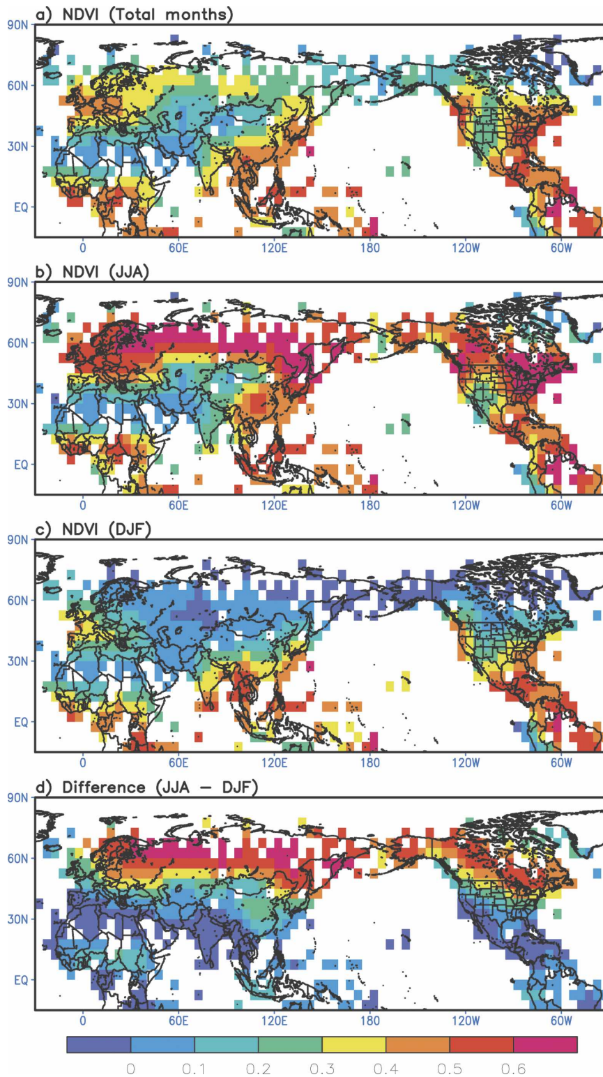
FIG. 2. Surface vegetation map derived from NDVI. Vegetation index is averaged over (a) 1981–94, (b) summer (JJA), and (c) winter (DJF). (d) The seasonal NDVI difference (JJA–DJF).
