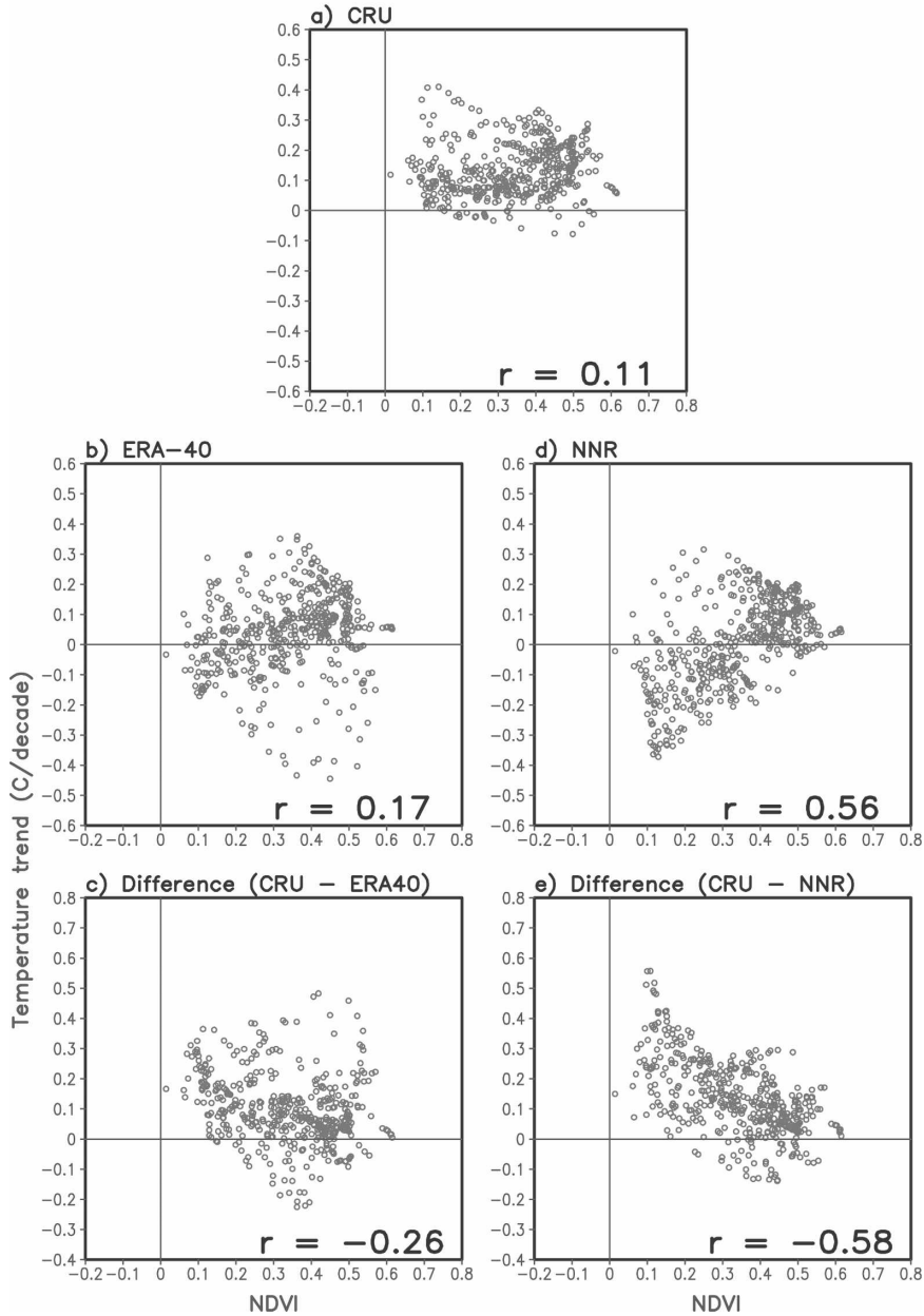
FIG. 4. As in Fig. 3 but for (a) CRU, (c) CRU-ERA-40, and (e) CRU-NNR.
