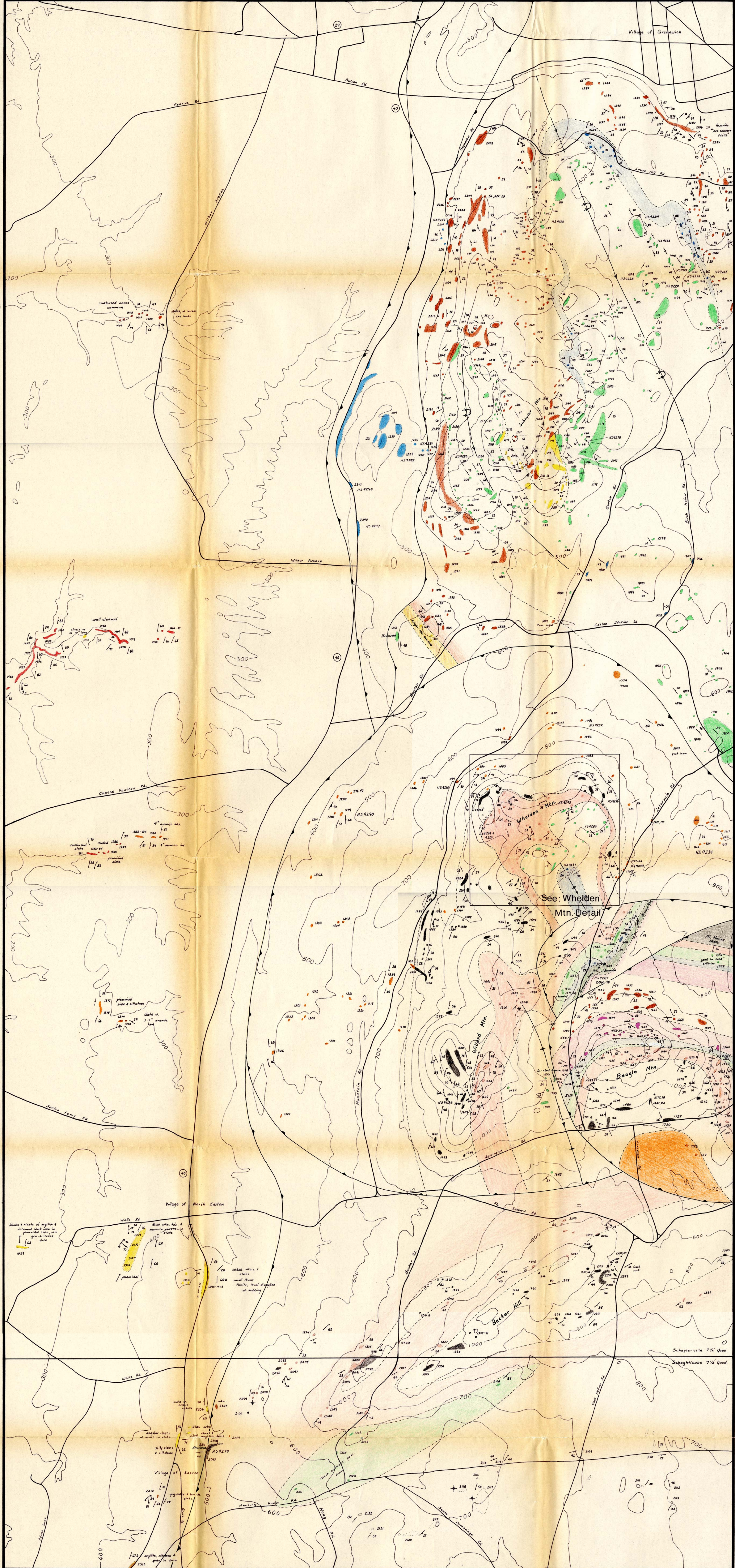
Plate 2 Geology of Schuyler & Willard Mtns.
