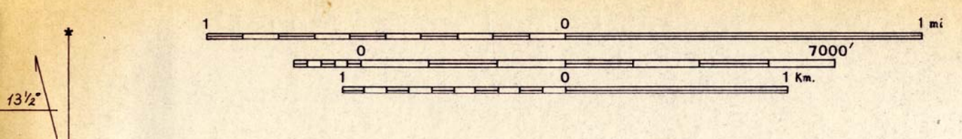
Plate 3 Geology of the Hudson River Lowlands FORT MILLER & SCHUYLerville 7 1/2' QUADRANGLES
