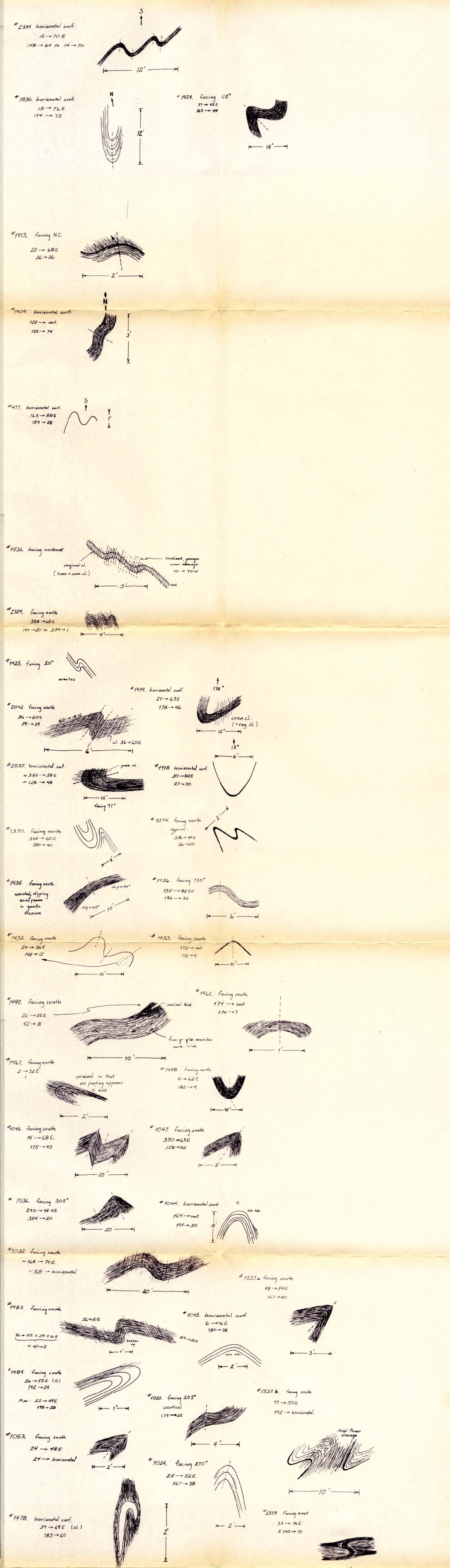
MESOSCOPIC FOLDS
