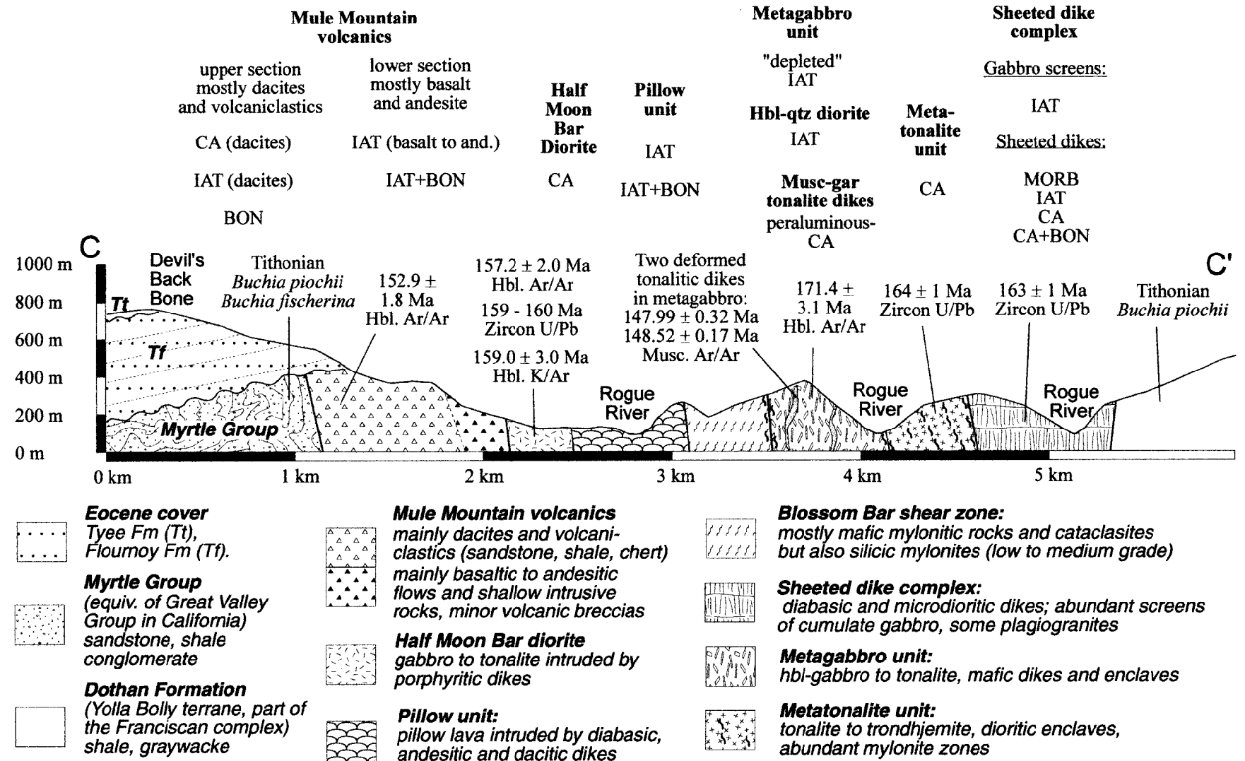
Figure 7.2: Cross section showing the units of the Wild Rogue Wilderness, sample ages and magmatic affinities.
