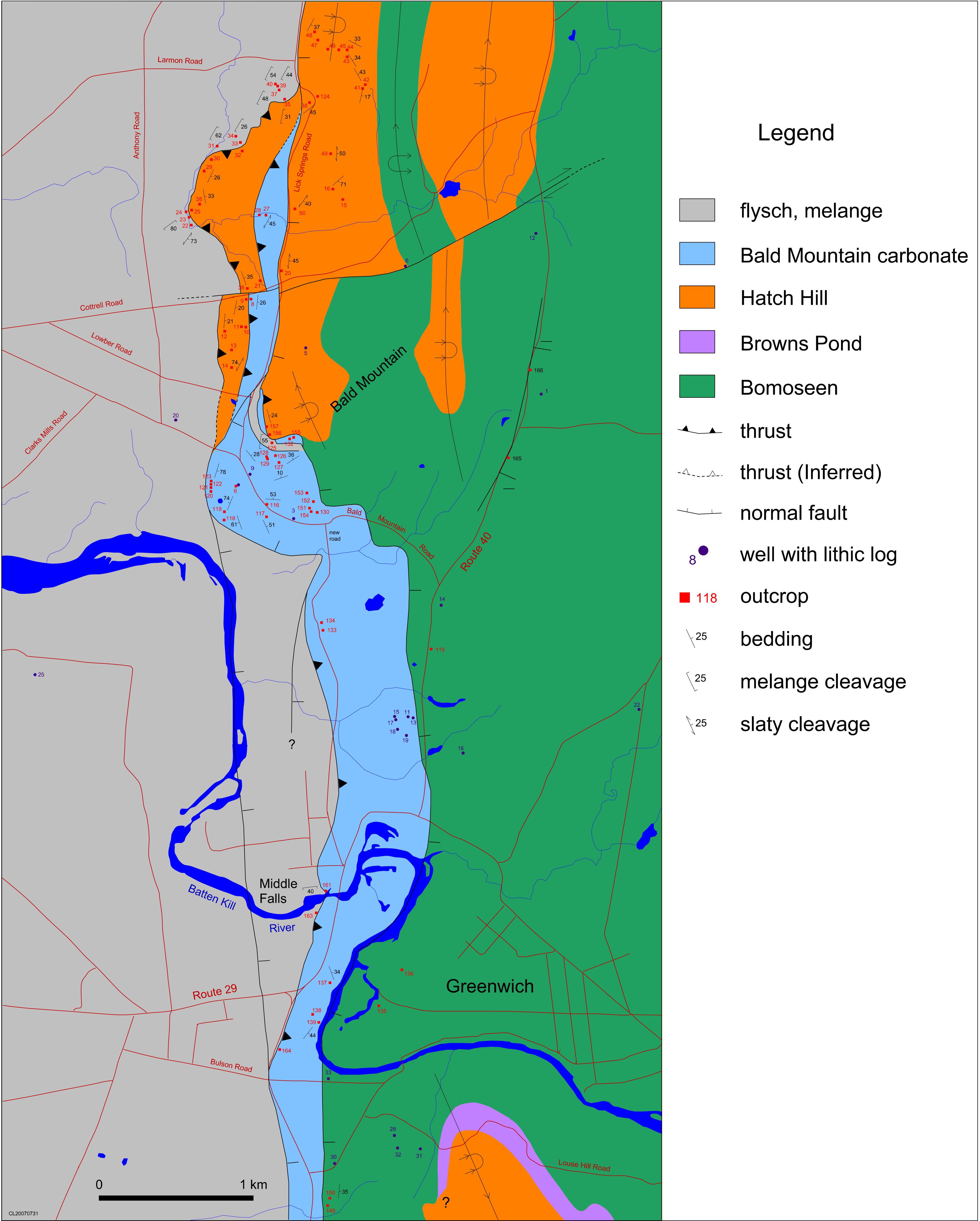
Plate 1. Geology of the Bald Mountain region, eastern New York (Chul Lim, 2007)
