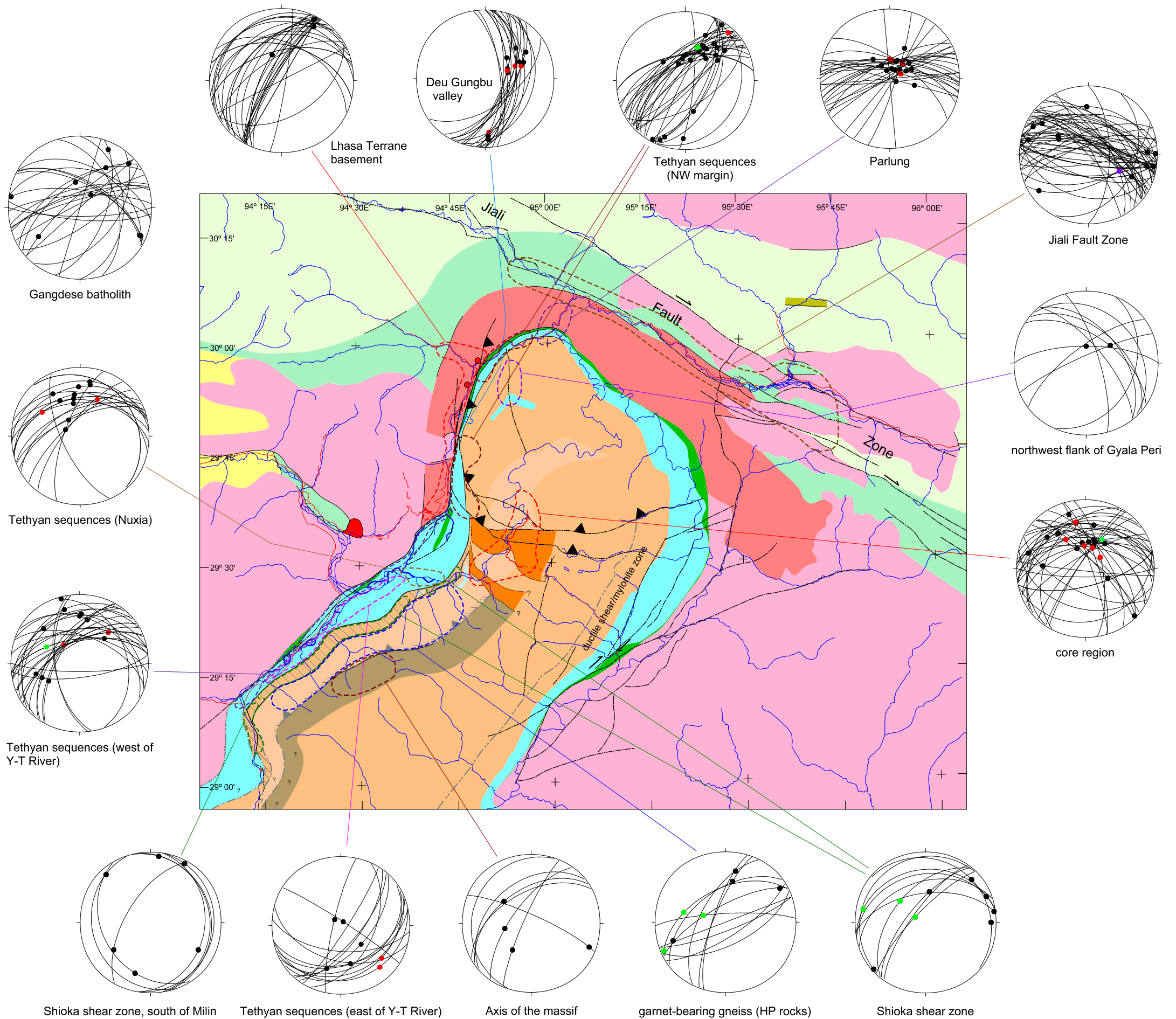
Plate 2. A map showing orientations of foliation and lineation in different localities. Lineations show shear senses of reverse (red), normal (green), or right-lateral (purple). Map compiled by W. S. F. Kidd from field observations of this project, Burg et al. (1997), and Geng et al. (2006).
