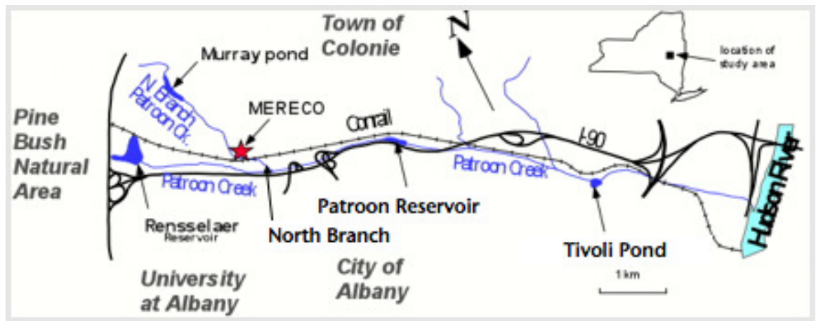
Figure 3. Map showing portions of the Patroon Creek watershed and sampling locations. Northerly pointing arrows show sample locations at North Branch, Patroon Reservoir, and Tivoli Pond. The red star shows the location of the Mereco point source. (Source: Fletcher, 2003)
