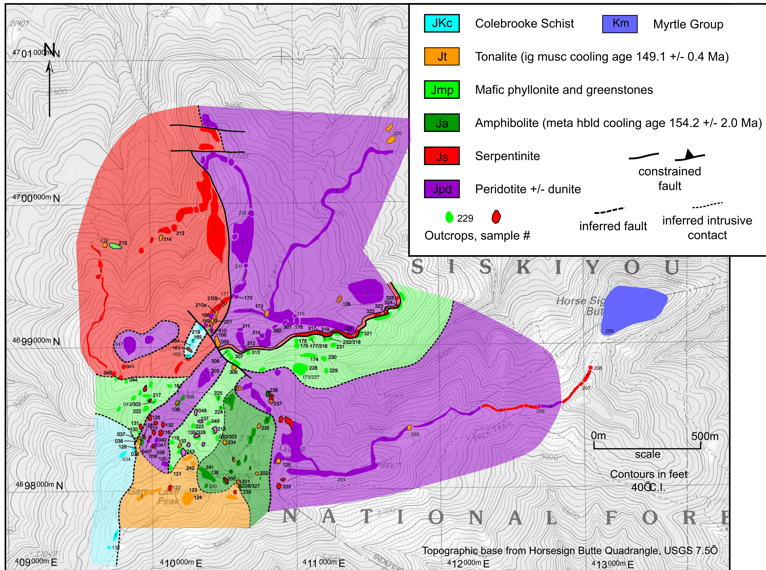
Plate 1. Geology of the Game Lake area, southwestern Oregon (Adam Schoonmaker, 2005)
