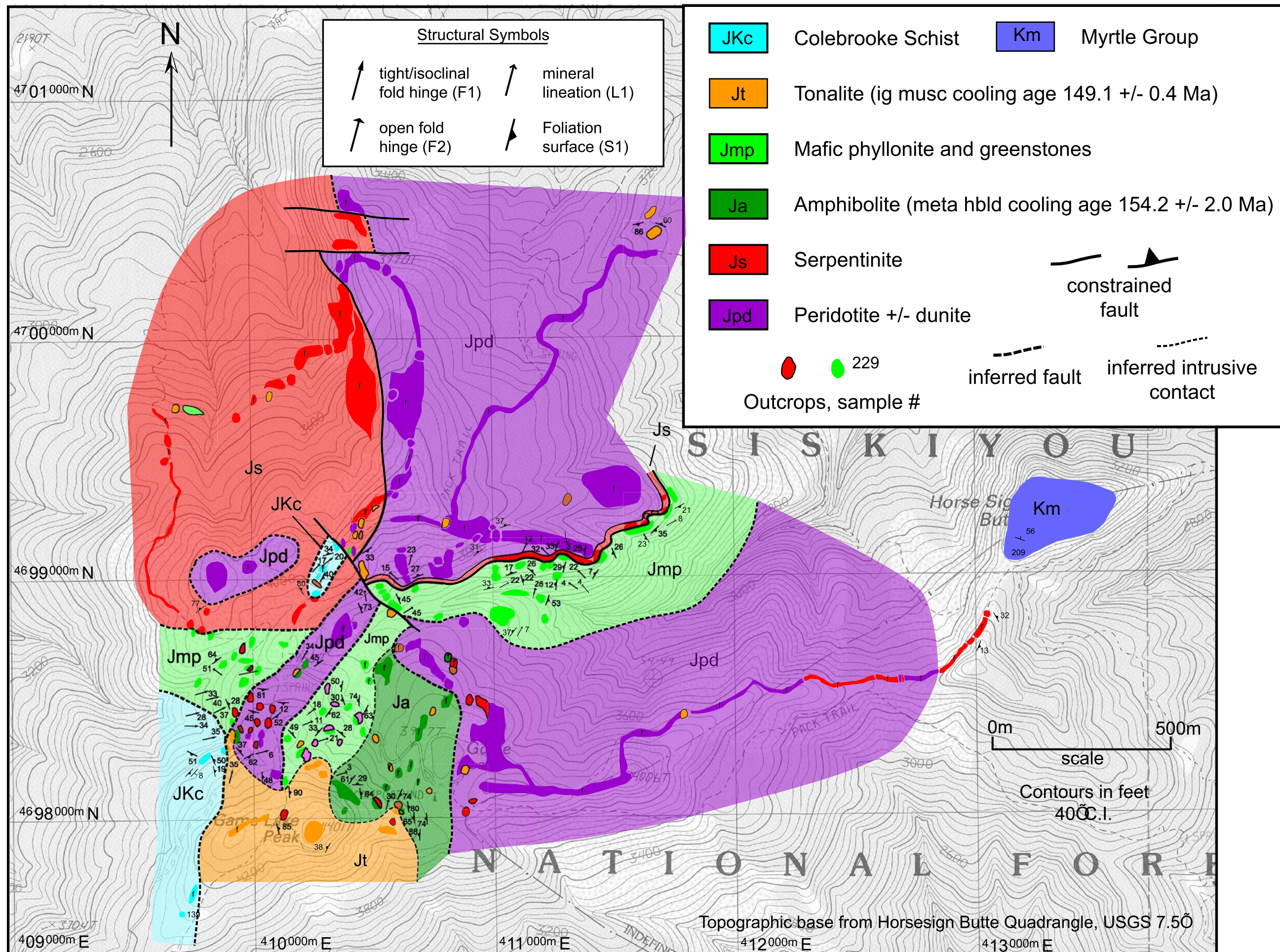
Plate 2. Geology and structure of the Game Lake area, southwestern Oregon (Adam Schoonmaker, 2005)
