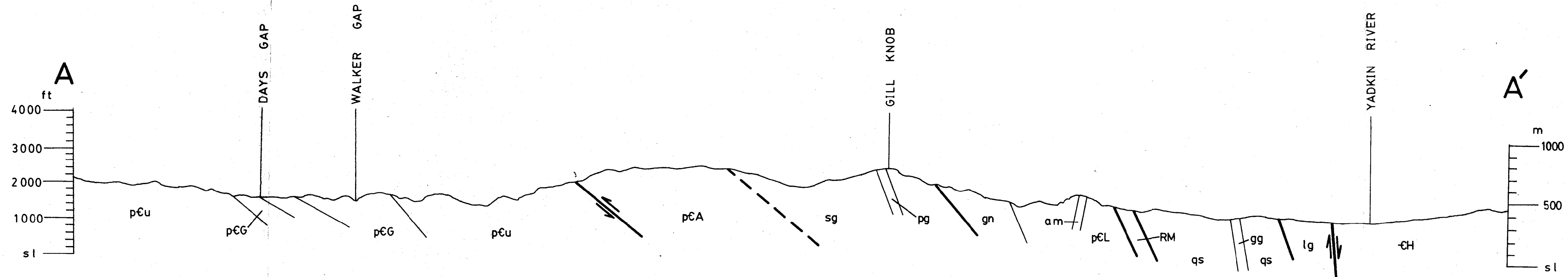
FIGURE 2-1D CROSS SECTION
