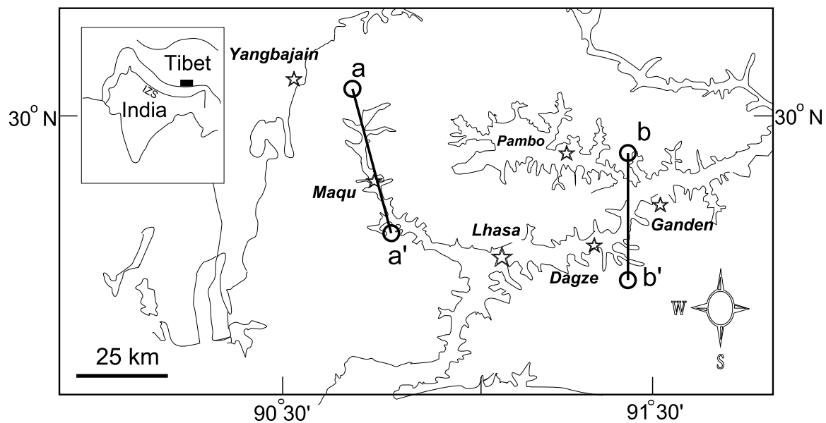
Locations of the Maqu cross section and the Dagze-Ganden cross section in the Lhasa area, southern Tibet.
