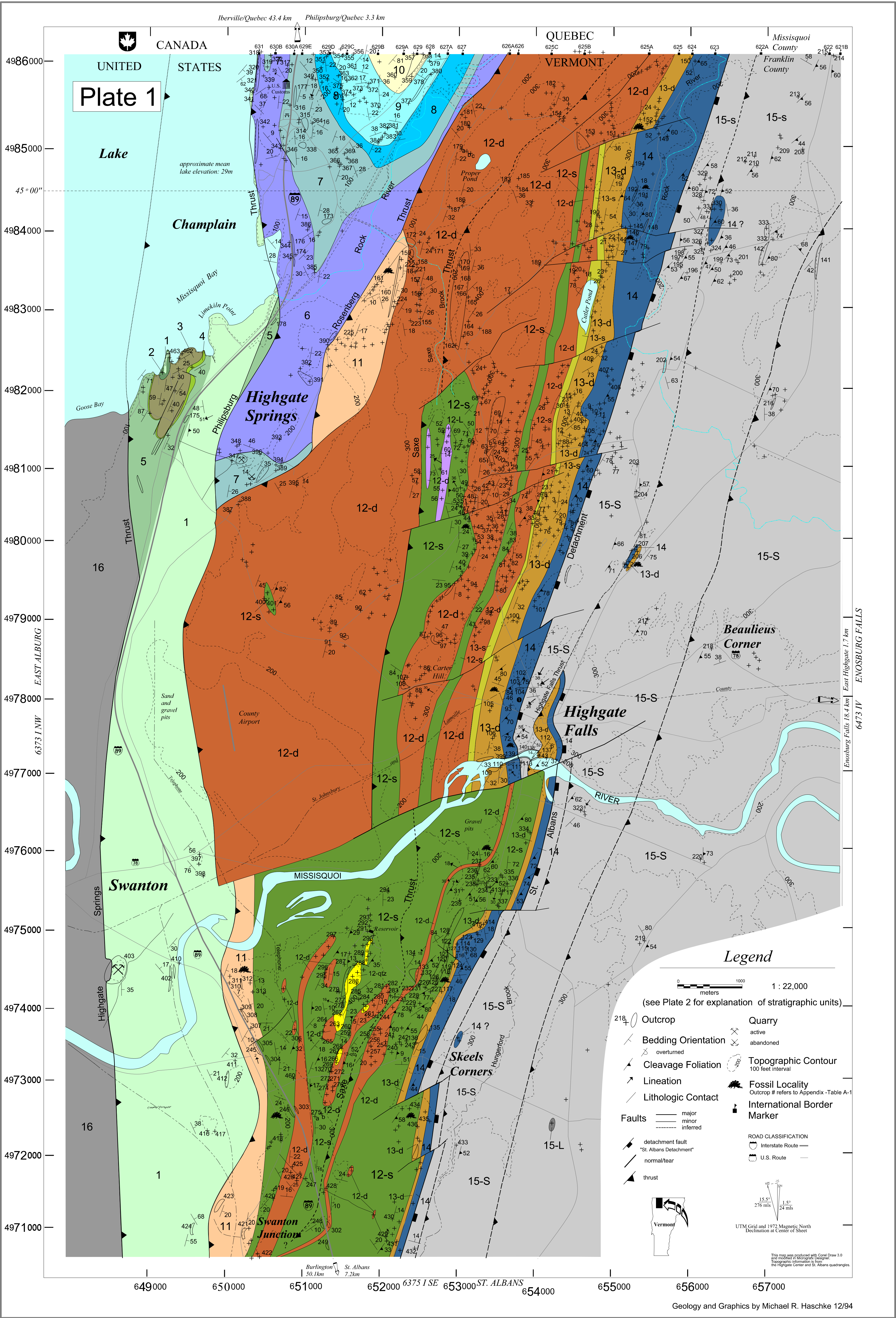
Lithostructural Units in the Highgate Center and St.Albans region, northwestern Vermont.
