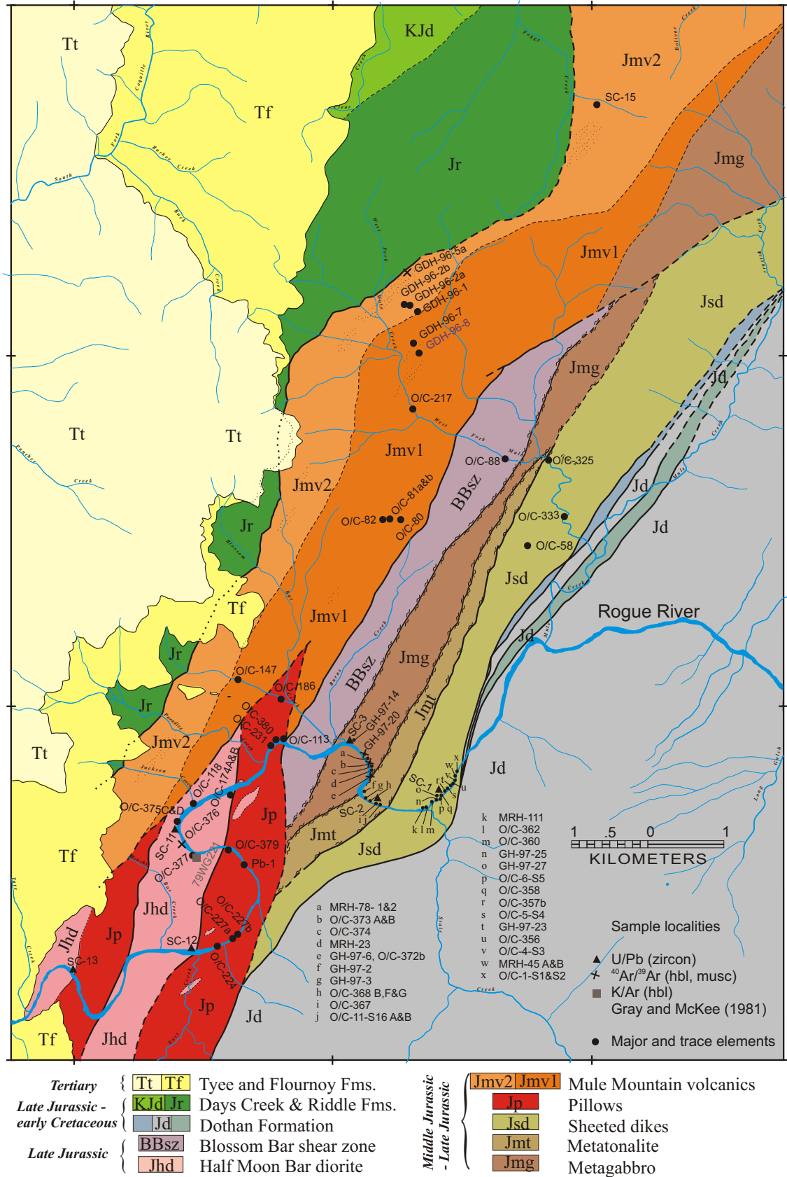
Figure 5.1: Simplified geologic map of the Wild Rogue Wilderness showing localities of analyzed samples.
