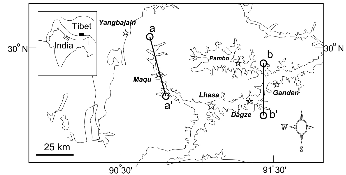
Locations of the Maqu cross section and the Dagze-Ganden cross section in the Lhasa area, southern Tibet.
