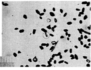
05-04a, U35Z-49 Grain 75
