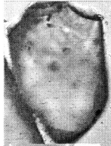
05-10a, U35Z-55 Grain 25
