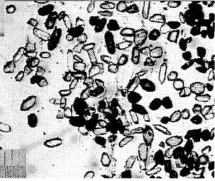
05-01b, U35Z-46 Grain 11
