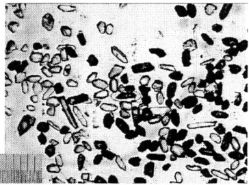
05-01b, U35Z-46 Grain 21
