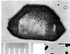
05-04a, U35Z-49 Grain 58
