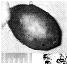
05-01b, U35Z-46 Grain 10
