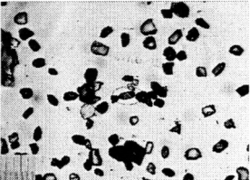
05-11a, U35Z-57 Grain 69
