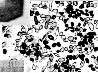
05-01b, U35Z-46 Grain 10
