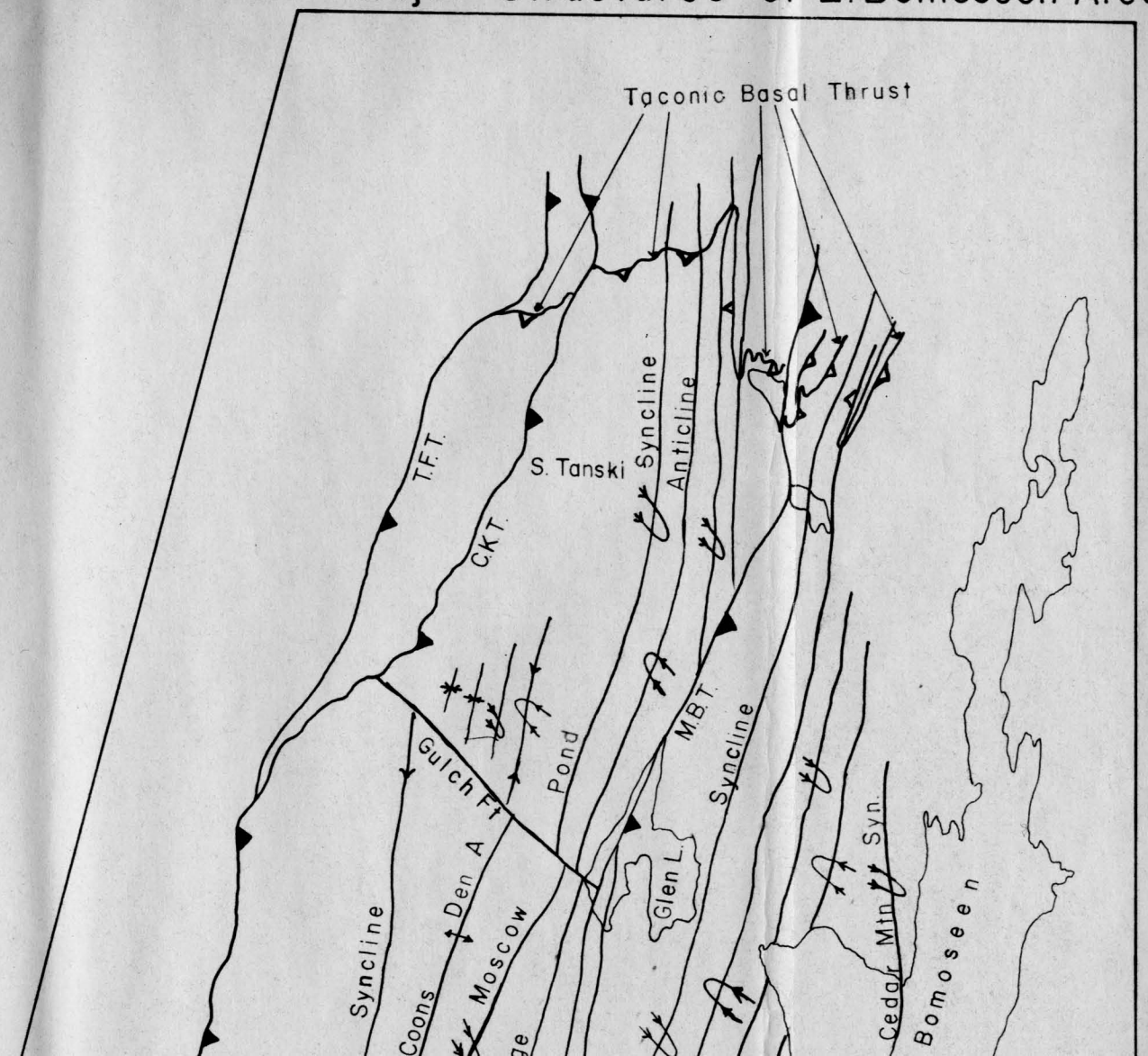
Major Structures of L. Bomoseen Area
