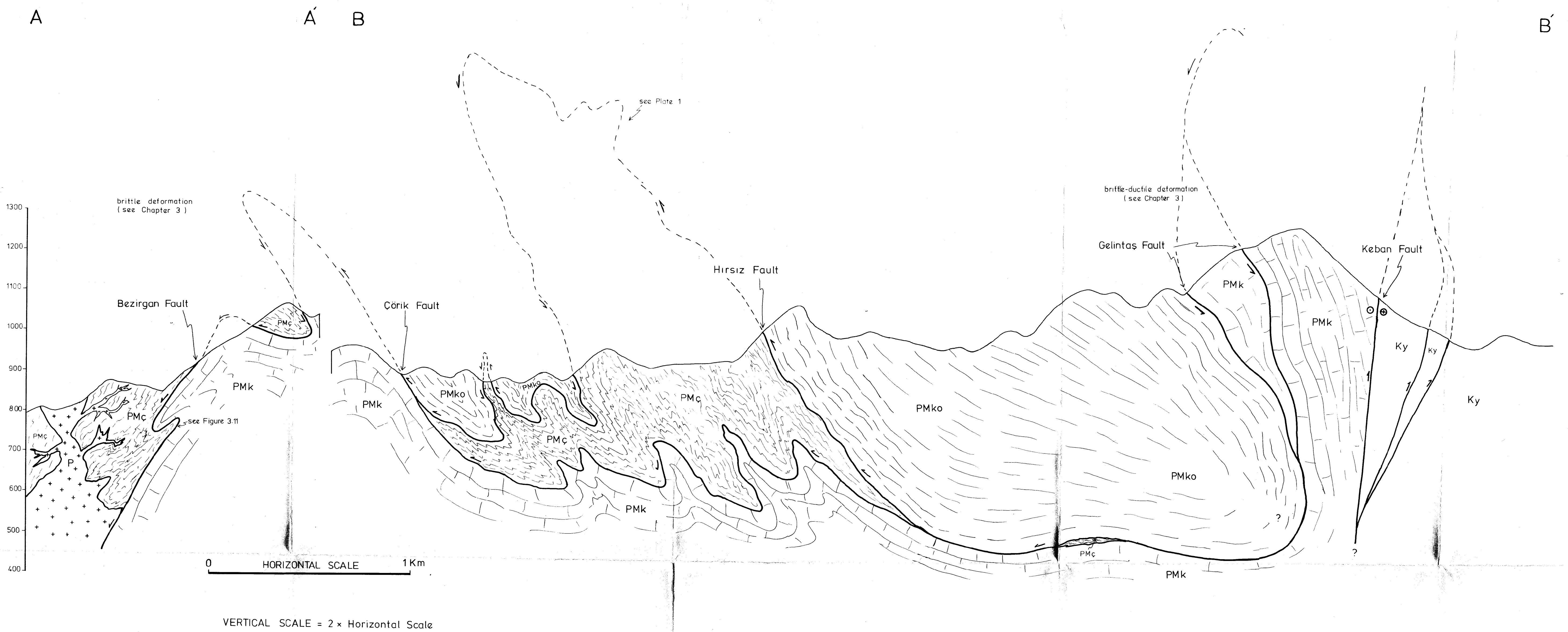
PLATE 2 GEOLOGICAL CROSS SECTION ( For geological signature see Plate 1 )
