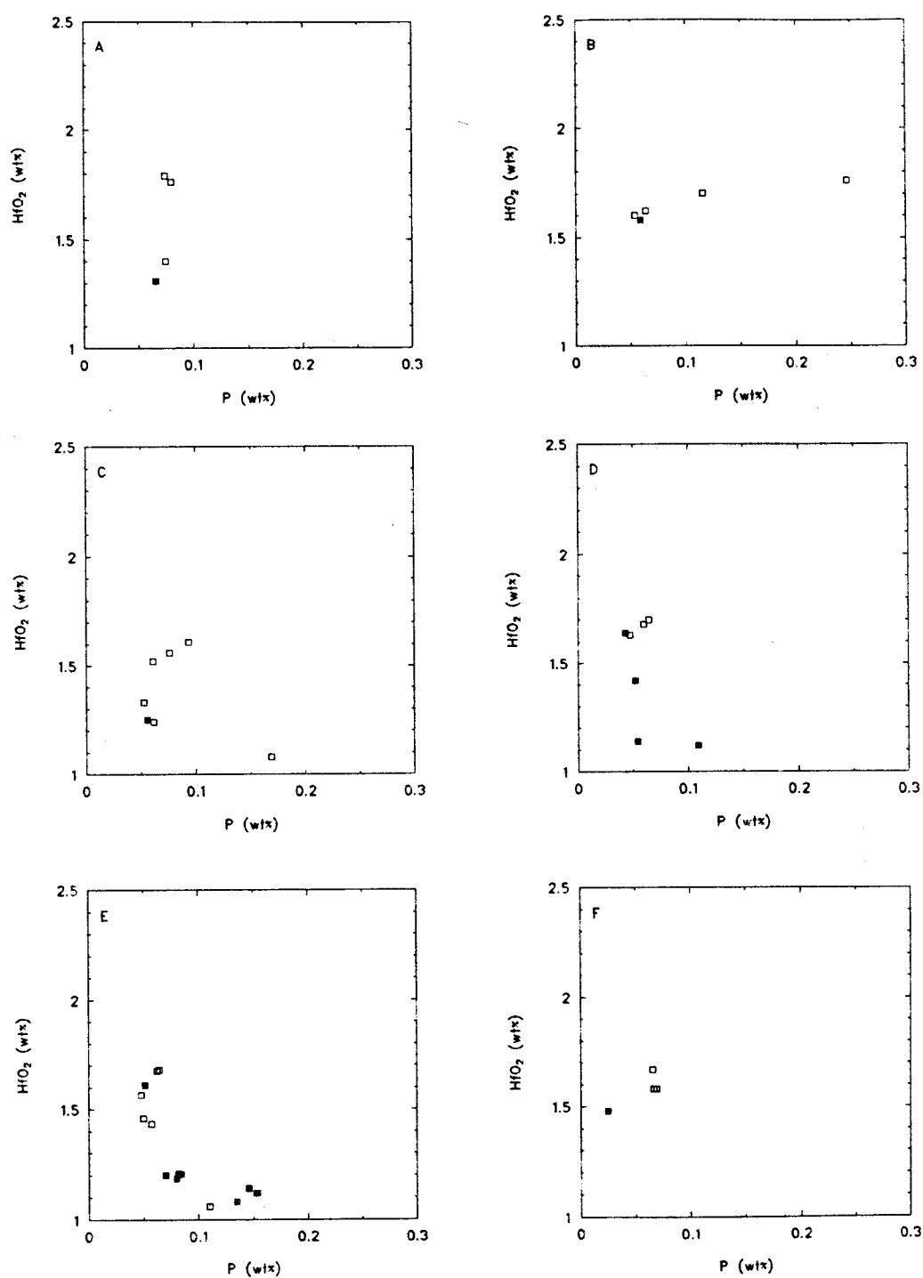
Figure 73: The variation of HfO 2 - and P-abundances within six individual grains from K-bentonite Can 14 (included in Figure 72). Analyses of cores are represented by filled boxes compared with open squares for rim analyses.
