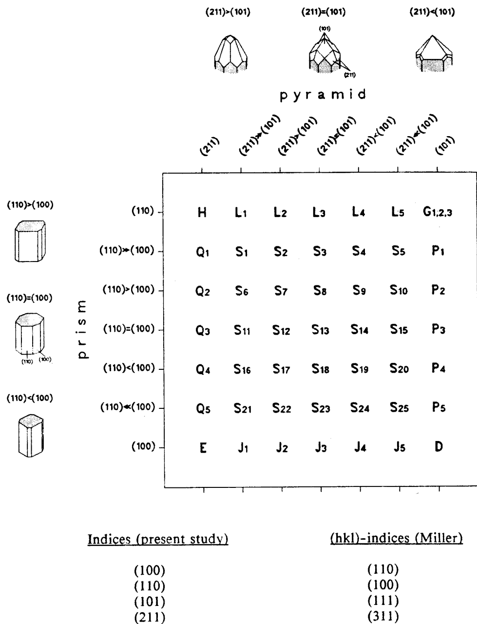
Figure 39: The classification scheme of zircon morphology (after Pupin and Turco, 1972b). Displayed are only the combinations of the two prism forms {100} and {110} with the pyramid forms {101} and {211}, which were observed among the zircon populations in the present study. The translation of the indices used for this scheme (after Caruba and Turco, 1971) to Miller (hkl)-indices is listed in the table.
