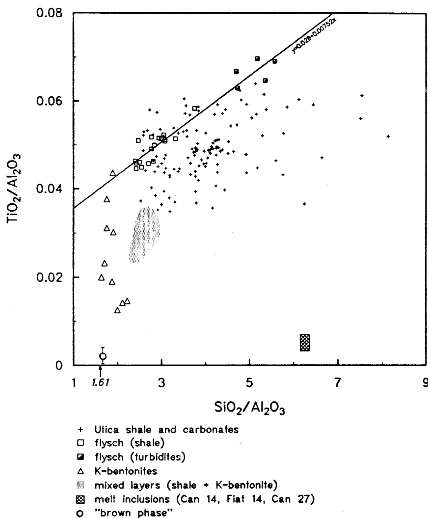
Figure 32: Plot of K-bentonites, shale samples and various lithologies of the flysch, illustrating the possible contamination of K-bentonites with \text{TiO}_2 -rich ( \text{Al}_2\text{O}_3 -normalized) mud particles of shale or flysch. Mixed layers of K-bentonite and shale are plotted for comparison. The line indicates the sorting trend of flysch sediments, such that \text{TiO}_2 increases relative to \text{Al}_2\text{O}_3 with increasing siliciclastic component (i.e. \text{SiO}_2/\text{Al}_2\text{O}_3 ratio).
