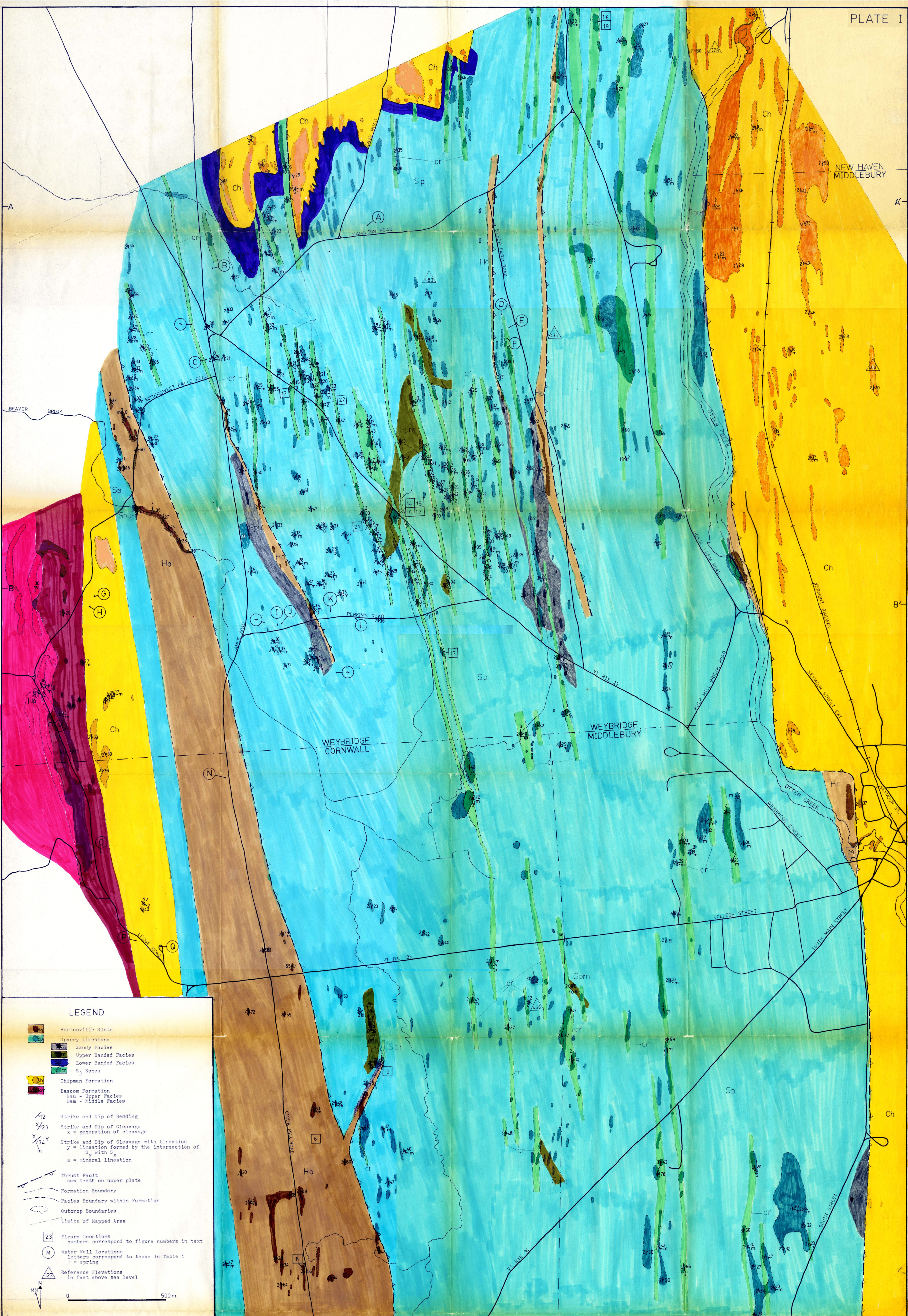
BEDROCK GEOLOGY NEAR MIDDLEBURY, VERMONT
